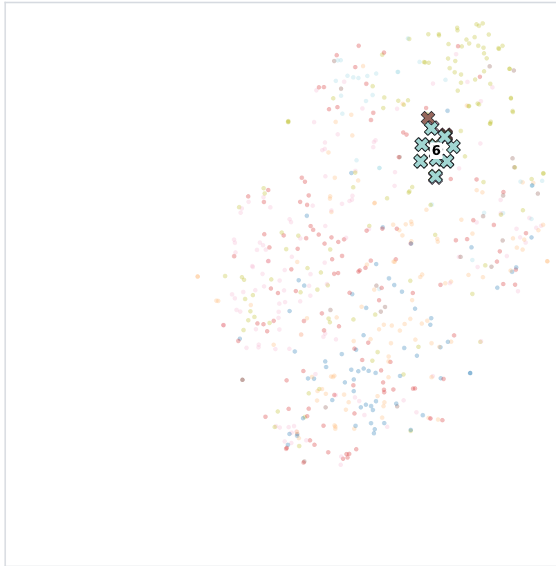
Global-feature mean
