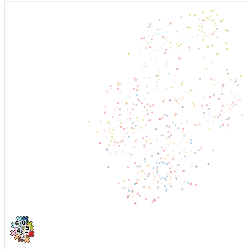
Classifier-head aggregation
