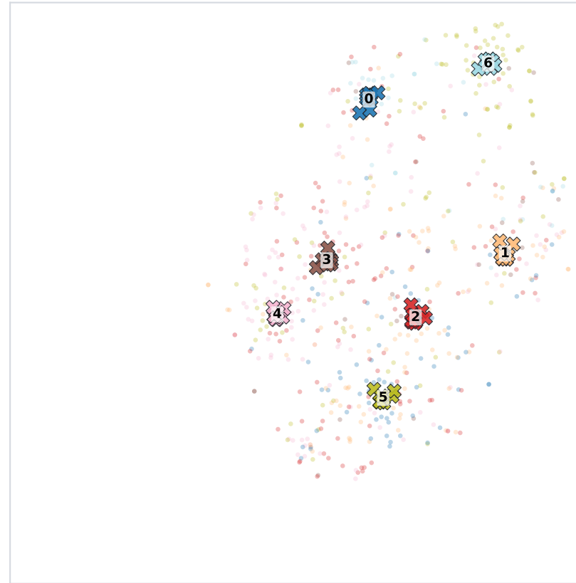
Shuffled-label prototype
