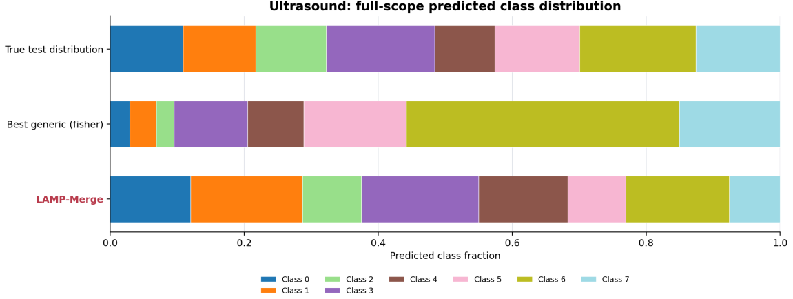
Figure 6: Predicted class distributions on Ultrasound. Each bar summarizes all formal settings for one prediction source; the generic merge concentrates predictions on one class, while LAMP-Merge recovers a broader class allocation aligned with the test distribution.
