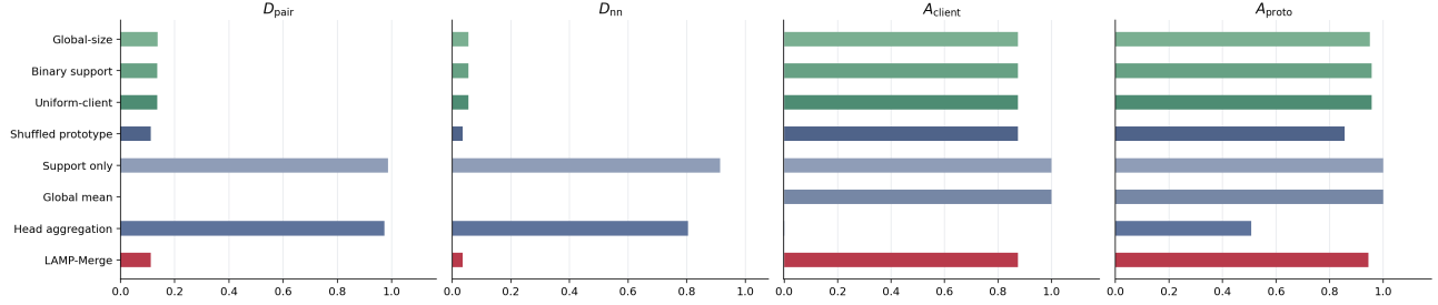
Figure 8: Prototype-geometry comparison on the full benchmark. The figure summarizes pairwise distance, nearest-class distance, prototype consistency, and prototype-client alignment.
