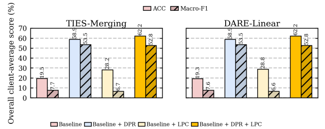
Figure 4: Strict 2 \times 2 DPR/LPC ablations for TIES-Merging and DARE-Linear. Each setting reports paired ACC and Macro-F1 bars. All experimental datasets are included.
