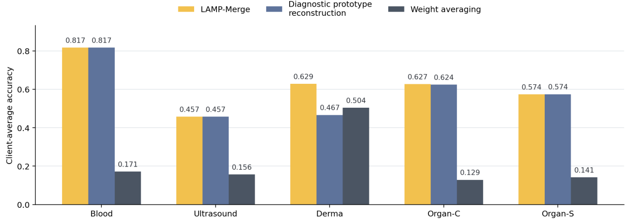
Figure 4: Dataset-level client-average accuracy in the module ablation. Each bar averages 12 client-average cells from four vision-model families and three client counts; every client-average cell is computed over three Dirichlet skew levels.
