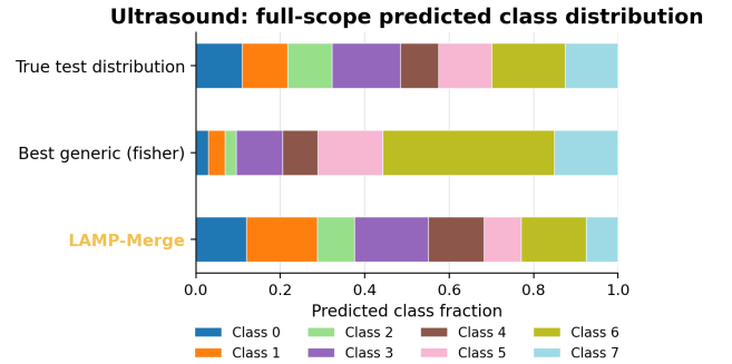
Figure 7: Predicted class distributions on Ultrasound, averaged over the four visual backbones, K \in \{3, 5, 7\} , and the three Dirichlet skew levels. The strongest generic reference (Fisher) concentrates predictions on a subset of classes, while LAMP-Merge recovers a broader allocation aligned with the test distribution.
