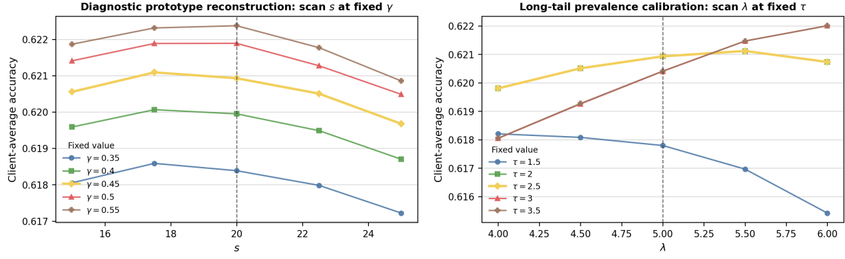
Figure 6: Full-scope hyperparameter sensitivity with five fixed-value curves per module. The formal settings s = 20 and \lambda = 5 lie in stable high-accuracy regions.
