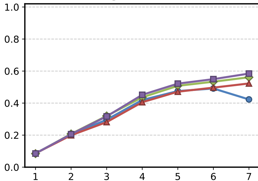
OrganSMNIST
