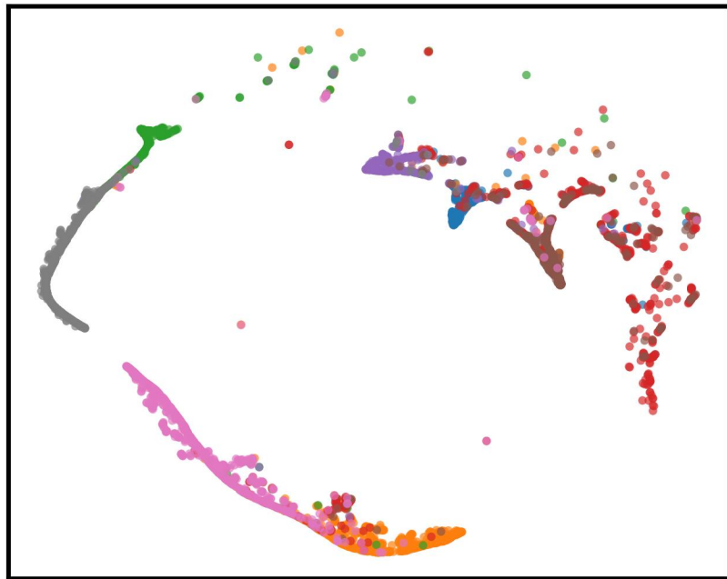
LAMP-Merge ACC=80.01%
