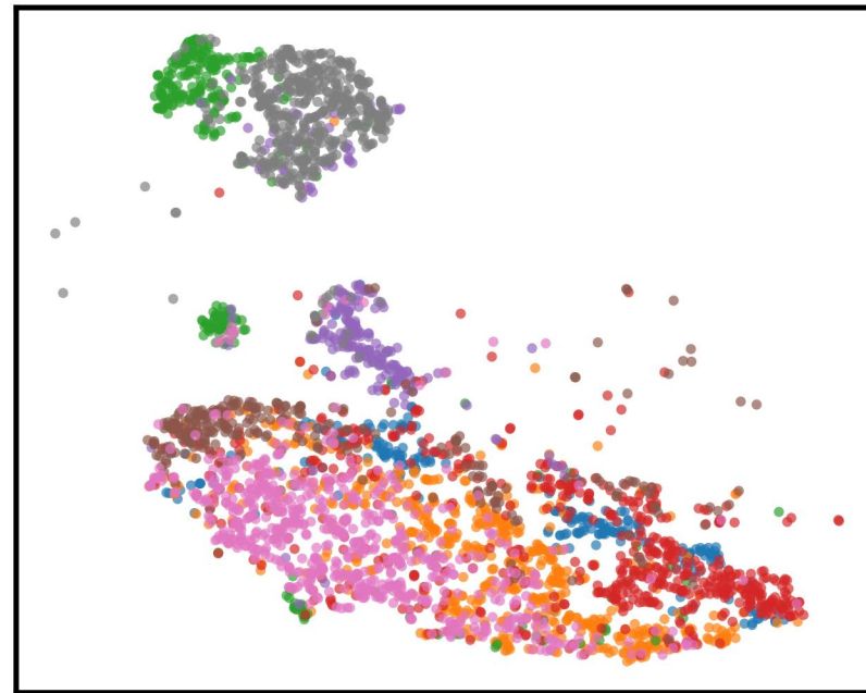
DARE-Linear ACC=33.76%
