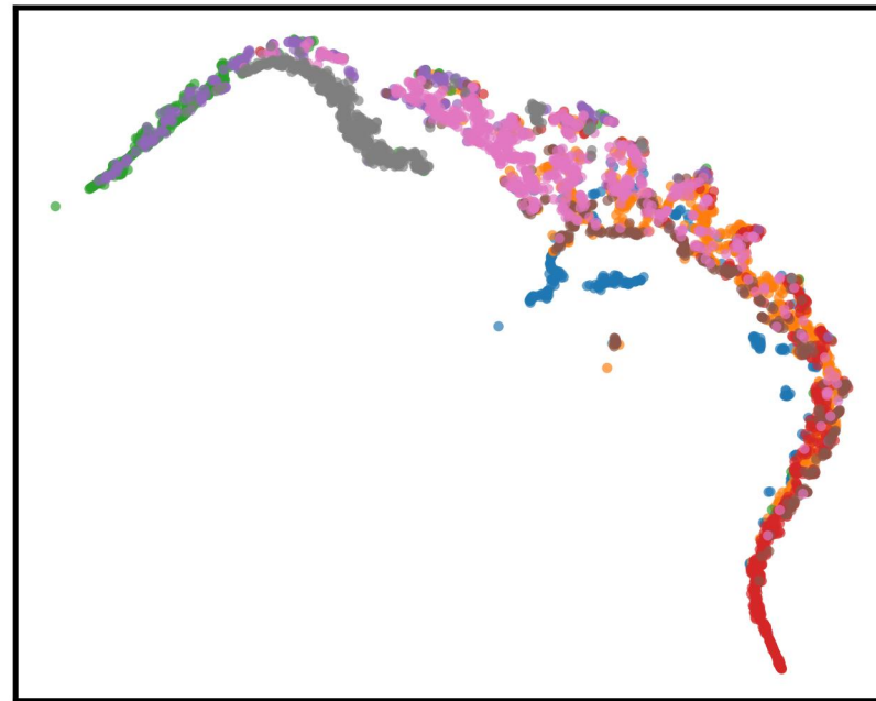
TIES-Merging ACC=27.97%
