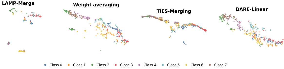
Figure 8: Joint t-SNE visualization of output-probability representations on Blood. From left to right: LAMP-Merge, weight averaging, TIES-Merging, and DARE-Linear.
