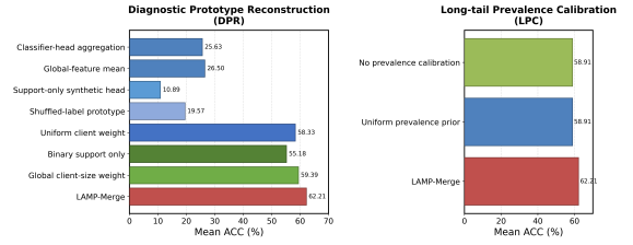
Figure 3: Internal ablations of the Diagnostic Prototype Reconstruction Module (DPR) and Long-tail Prevalence Calibration (LPC).
