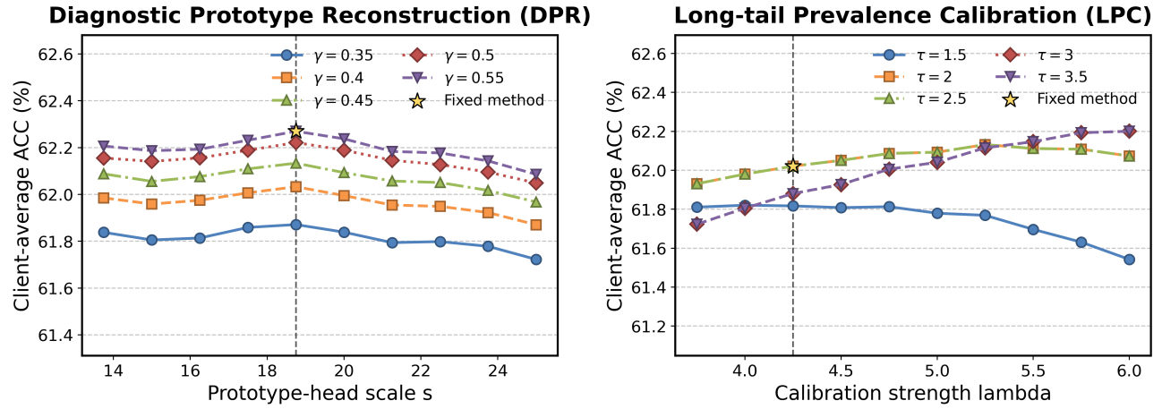
Figure 6: Full-scope hyperparameter sensitivity for DPR and LPC. The expanded vertical ranges emphasize that accuracy remains stable across broad parameter intervals.
