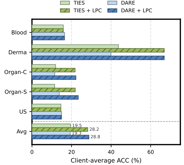
Figure 4: Strict 2 \times 2 baseline ablation over TIES- and DARE-merged classifier heads, with LPC disabled or enabled. DPR is disabled in all four settings. Each dataset bar averages 12 client-average cells, and Avg averages all 60 cells.
