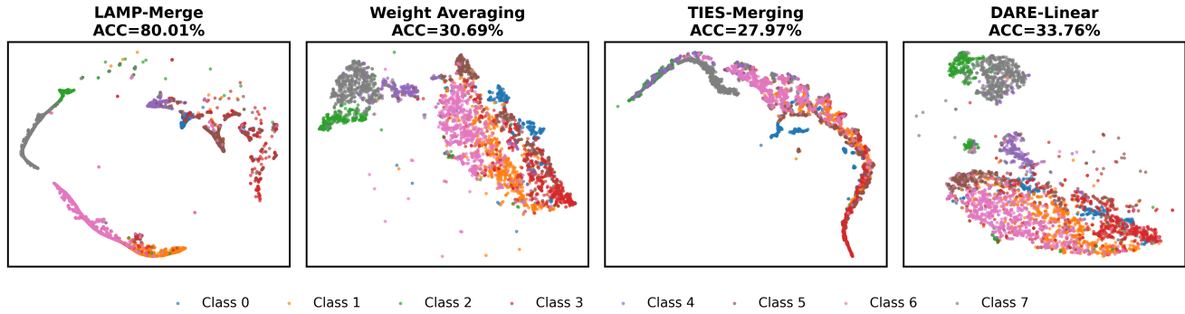
Figure 7: Joint t-SNE of test-image output-probability representations on Blood; from left to right, LAMP-Merge, weight averaging, TIES-Merging, and DARE-Linear.
