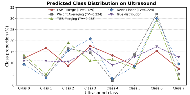
Figure 5: Predicted class distributions on Ultrasound, averaged over the four visual backbones, K \in \{3, 5, 7\} , and the three Dirichlet skew levels. Generic merges concentrate predictions on a few classes, while LAMP-Merge recovers a broader class allocation aligned with the test distribution.
