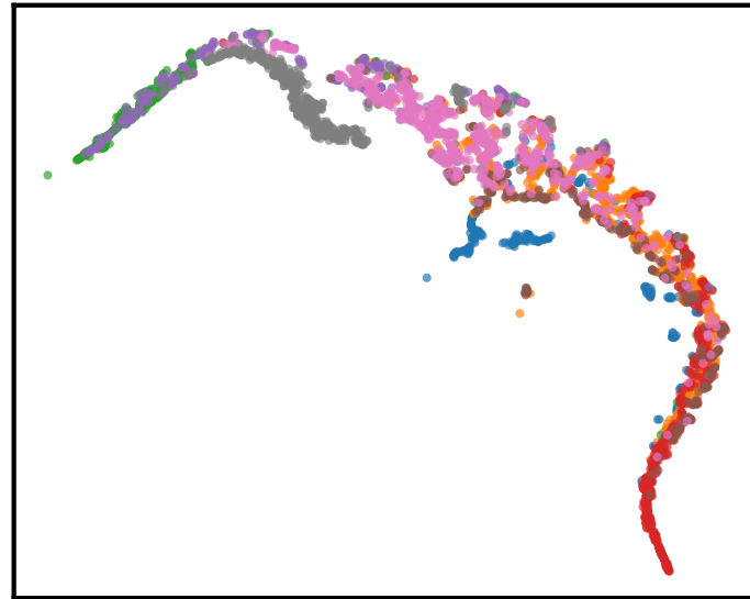
TIES-Merging ACC=27.97%
