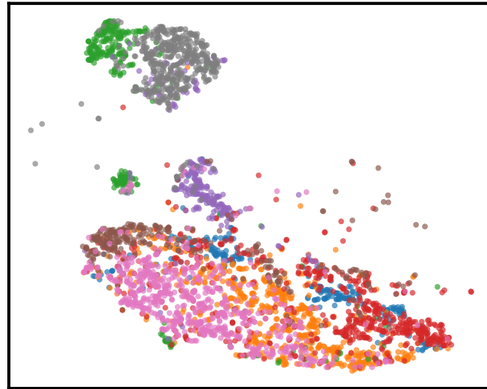
DARE-Linear ACC=33.76%
