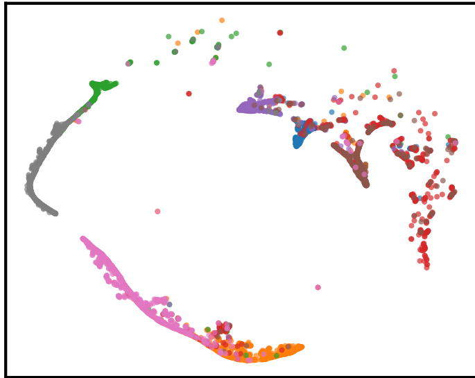
LAMP-Merge ACC=80.01%
