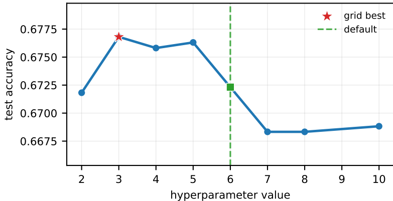
M2: long-tail bias strength
