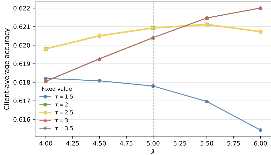
Long-tail prevalence calibration: scan \lambda at fixed \tau
