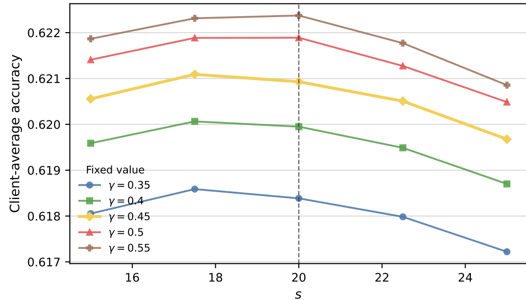
Diagnostic prototype reconstruction: scan s at fixed \gamma
