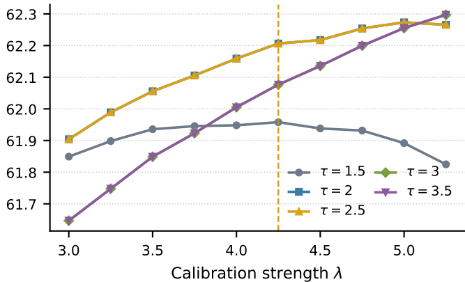
Long-tail Prevalence Calibration
