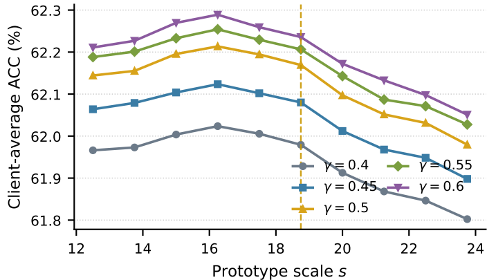
Diagnostic Prototype Reconstruction
