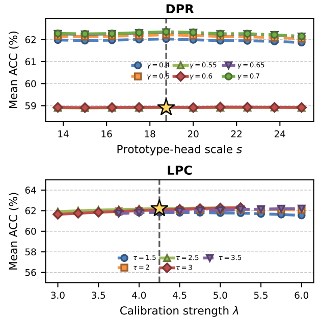
Figure 6: Full-scope DPR and LPC sensitivity. Solid curves use the 2026-07-19 grid; dashed and dash-dotted curves use earlier complete grids. Each point averages 60 client-average cells.
