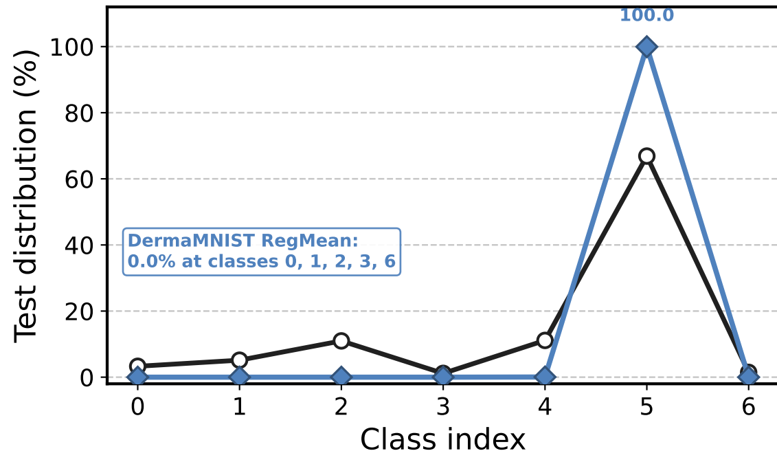
Medical DermaMNIST
