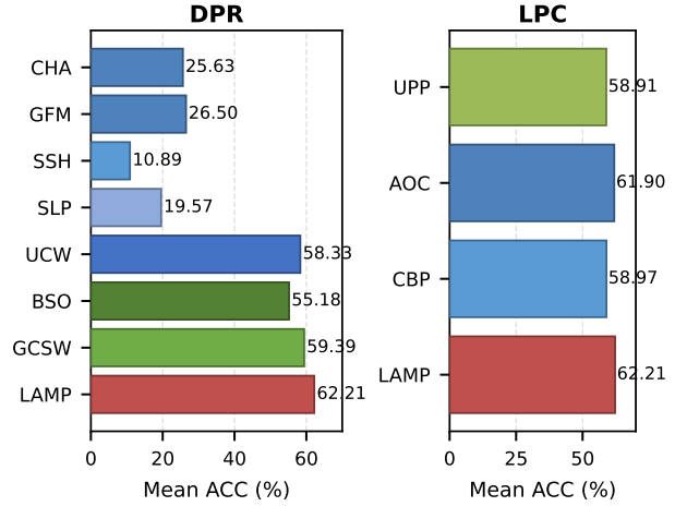
Figure 3: Internal ablations of the Diagnostic Prototype Reconstruction (DPR) and Long-tail Prevalence Calibration (LPC) modules. Full names and configurations of the plotted abbreviations are provided in the supplementary ablation configurations.
