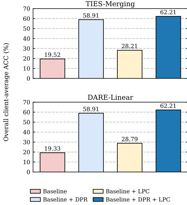
Figure 4: Strict 2 \times 2 DPR/LPC ablations for TIES-Merging and DARE-Linear. Values are overall ACC across 60 client-average cells (five datasets, four backbones, and three client counts).
