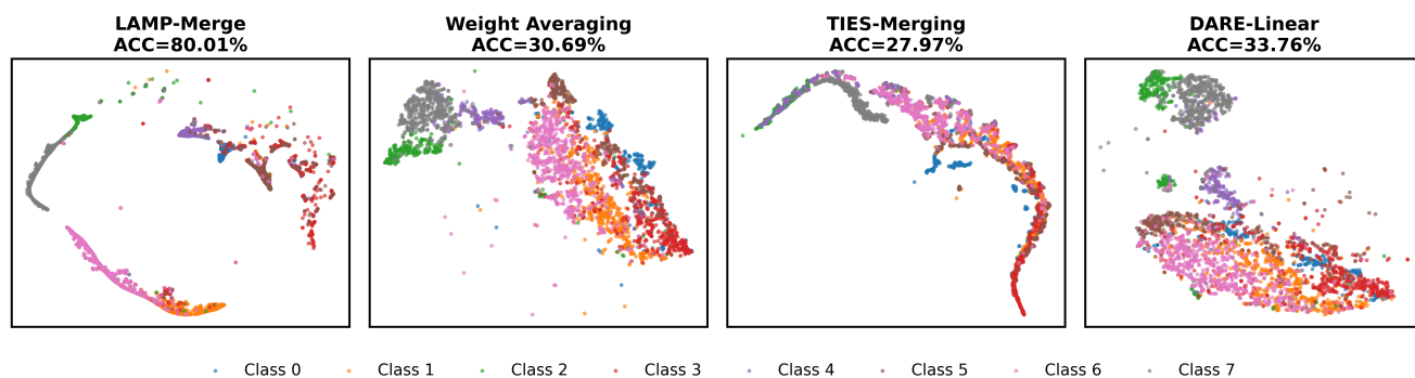
Figure 7: Joint t-SNE of test-image output-probability representations on Blood; from left to right, LAMP-Merge, weight averaging, TIES-Merging, and DARE-Linear.
