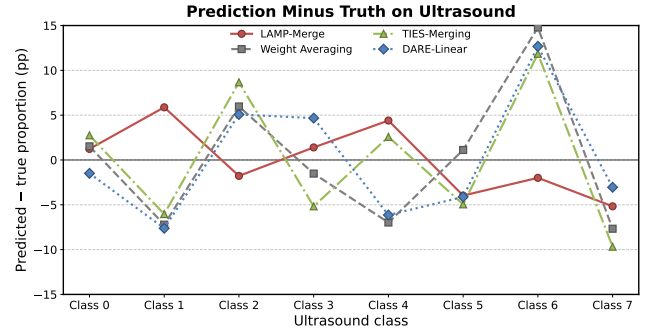
Figure 5: Per-class prediction deviations on Ultrasound, averaged over the four visual backbones, K \in \{3, 5, 7\} , and the three Dirichlet skew levels. Values are predicted minus true class proportions in percentage points; zero denotes exact distributional agreement.
