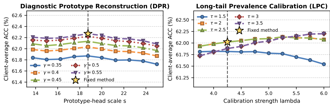
Figure 6: Full-scope hyperparameter sensitivity of DPR and LPC. Expanded vertical ranges show stable accuracy across broad intervals.
