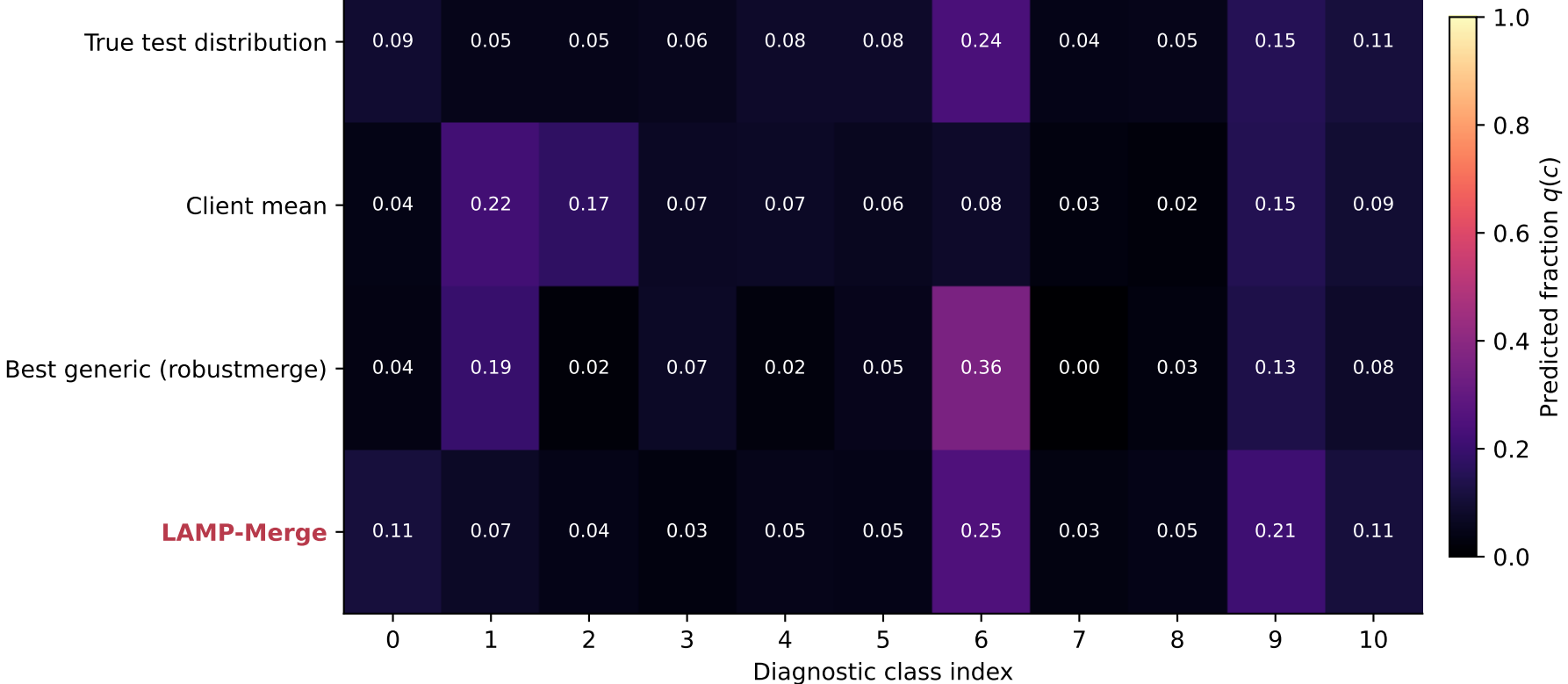
Organ-S: full-scope predicted class distribution
