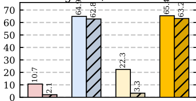
Organ-C / ConvNeXt
