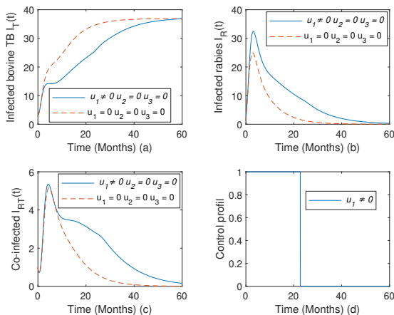
Figure 4: Effects of vaccination control on bovine TB, rabies and the co-infection transmission dynamics, with \alpha = 0.995
