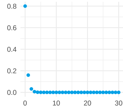
r = 1, p = 0.8
