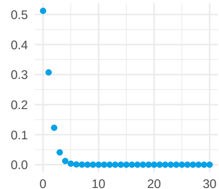
r = 3, p = 0.8
