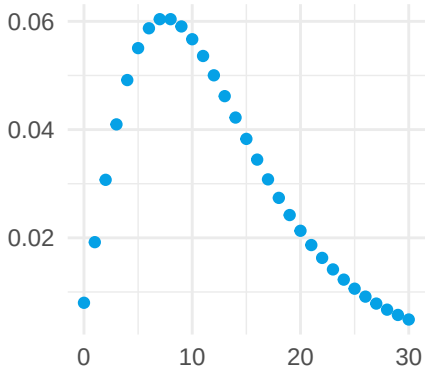
r = 3, p = 0.5
