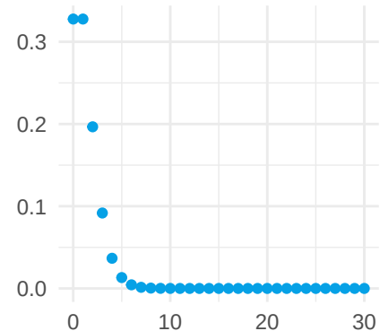
r = 5, p = 0.8
