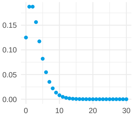
r = 3, p = 0.8
