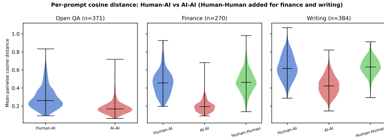
Fig. 2. Per-prompt pairwise cosine distances. Blue: mean Human–AI; red: mean AI–AI; green (finance and writing): mean Human–Human, on prompts with \geq 2 human answers (270 finance, 384 writing; all violins in a panel use that subset). AI–AI is below Human–AI in all three domains (87–98% of prompts) and below Human–Human on 97.8% of finance and 94.3% of writing prompts. The QA panel has no Human–Human violin (HC3 gives one human per prompt). Distances are cross-model: two users querying different developers’ models get answers closer to each other than to a human.
