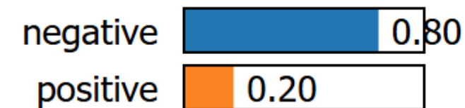
Prediction probabilities
