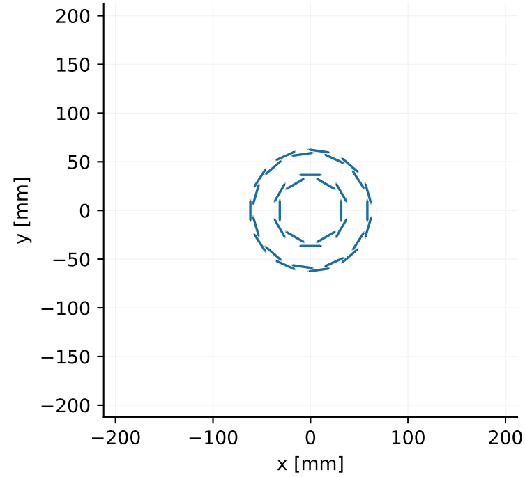
Pixels · z = 24.40 mm 82 bodies / 82 sensor cuts
