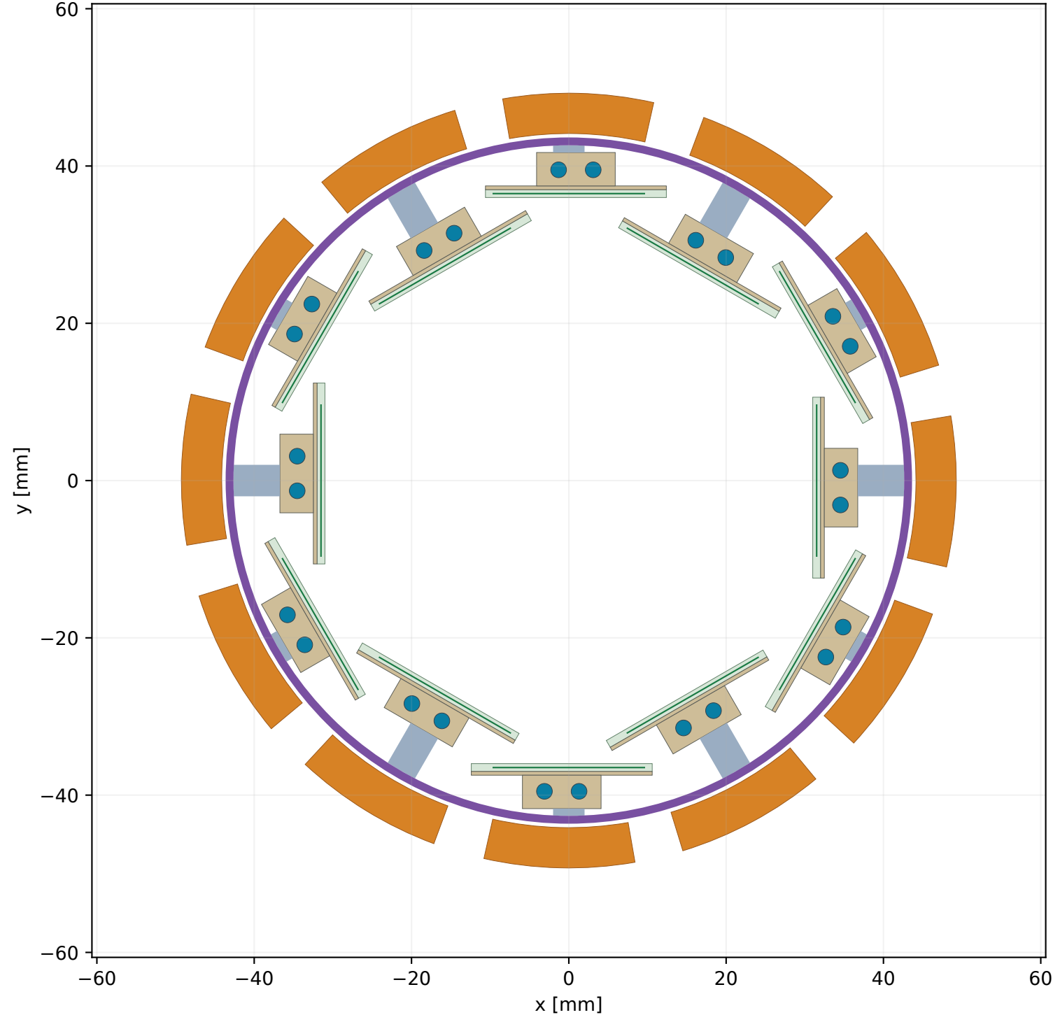
Candidate A | B1 | actual x-y cut at z = +110 mm Cumulative electrical bundles outside mounting rings
