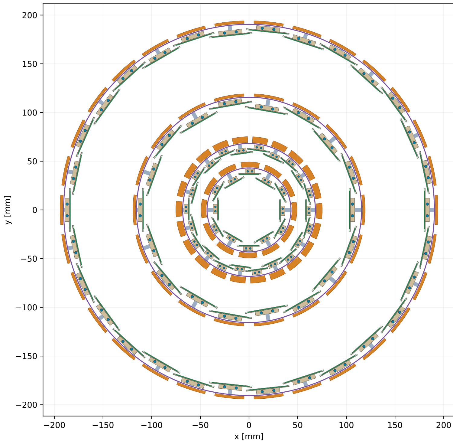
Candidate A | all | actual x-y cut at z = +110 mm Cumulative electrical bundles outside mounting rings
