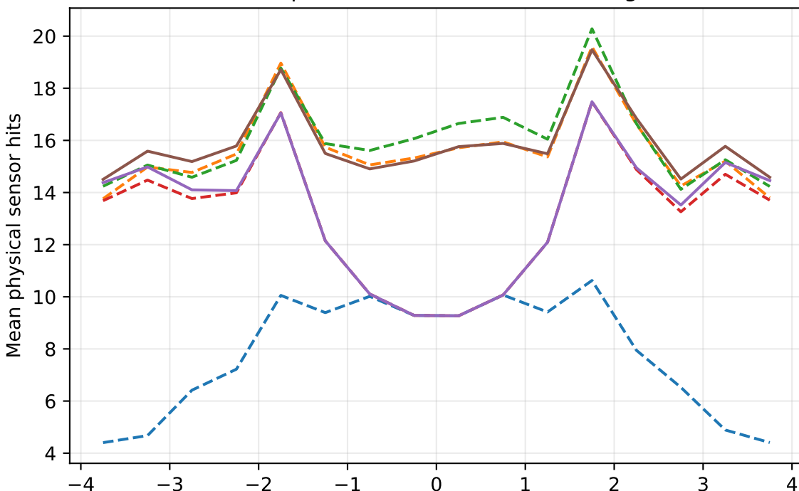
cobe: pT = 1 GeV, B_z = 3 T, + charge
