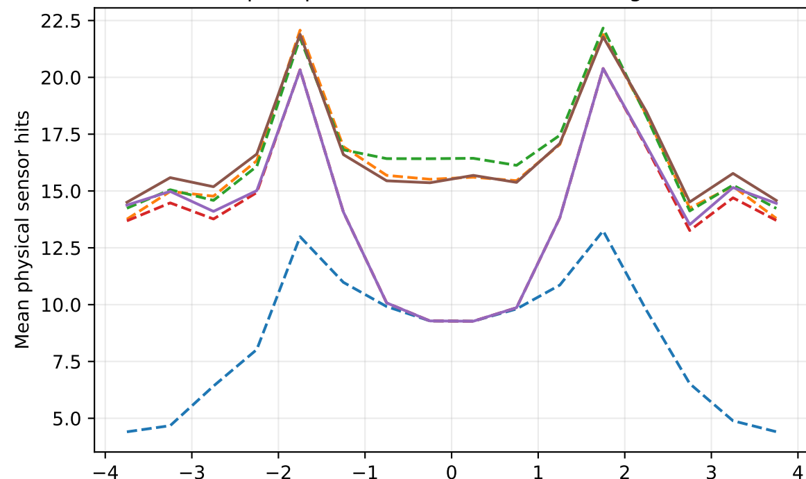
pint: pT = 1 GeV, B_z = 3 T, + charge
