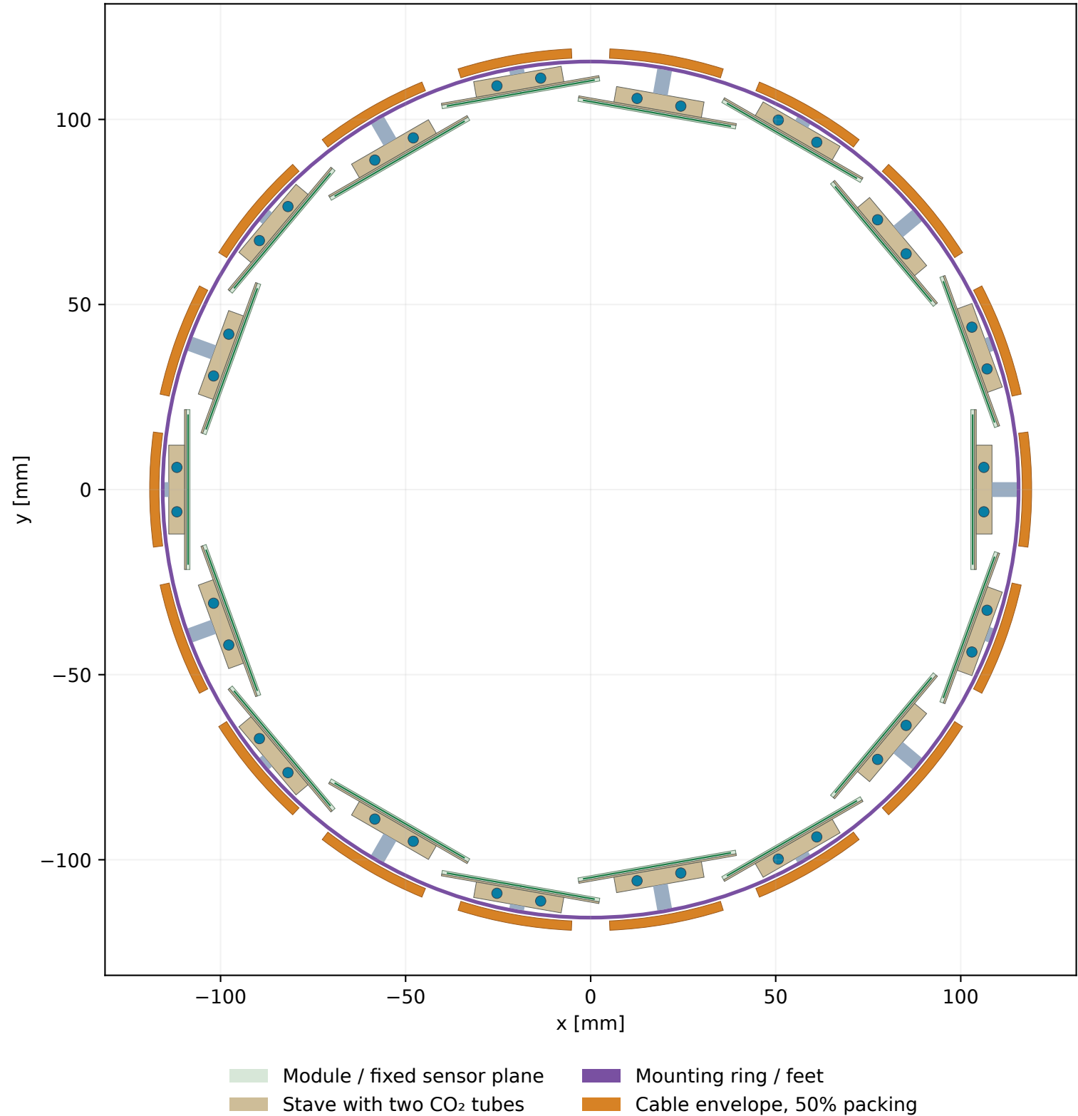
Candidate A | B3 | actual x-y cut at z = +110 mm Cumulative electrical bundles outside mounting rings
