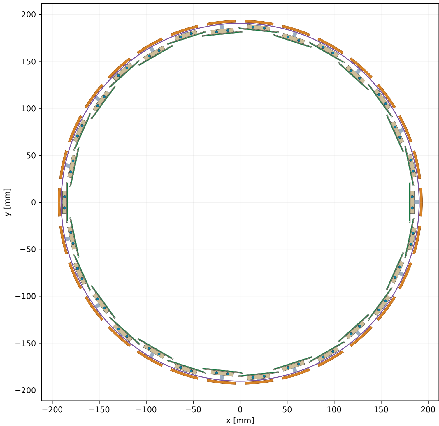
Candidate A | B4 | actual x-y cut at z = +110 mm Cumulative electrical bundles outside mounting rings
