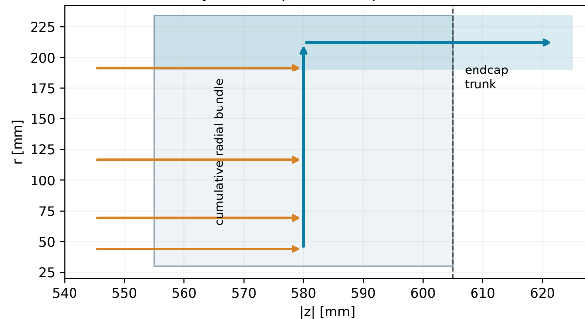
Radial bay \rightarrow outer pixel endcap trunk (schematic)
