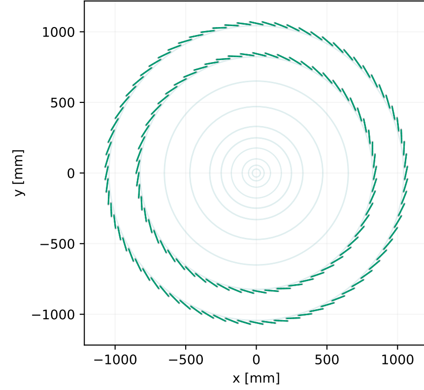
Long-strip pairs · first disc projection Nominal z = 1466.65 mm
