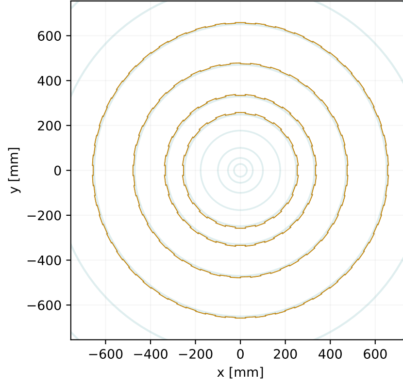
Short strips · first disc projection Nominal z = 1295.5 mm
