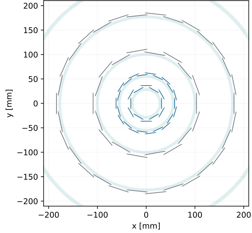
Pixels · first disc projection Nominal z = 611.7 mm
