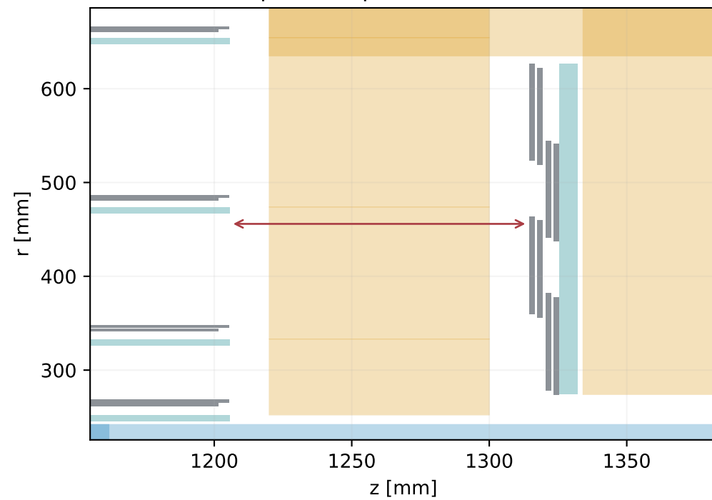
Short strips · barrel / first disc Occupied z separation: 109.00 mm
