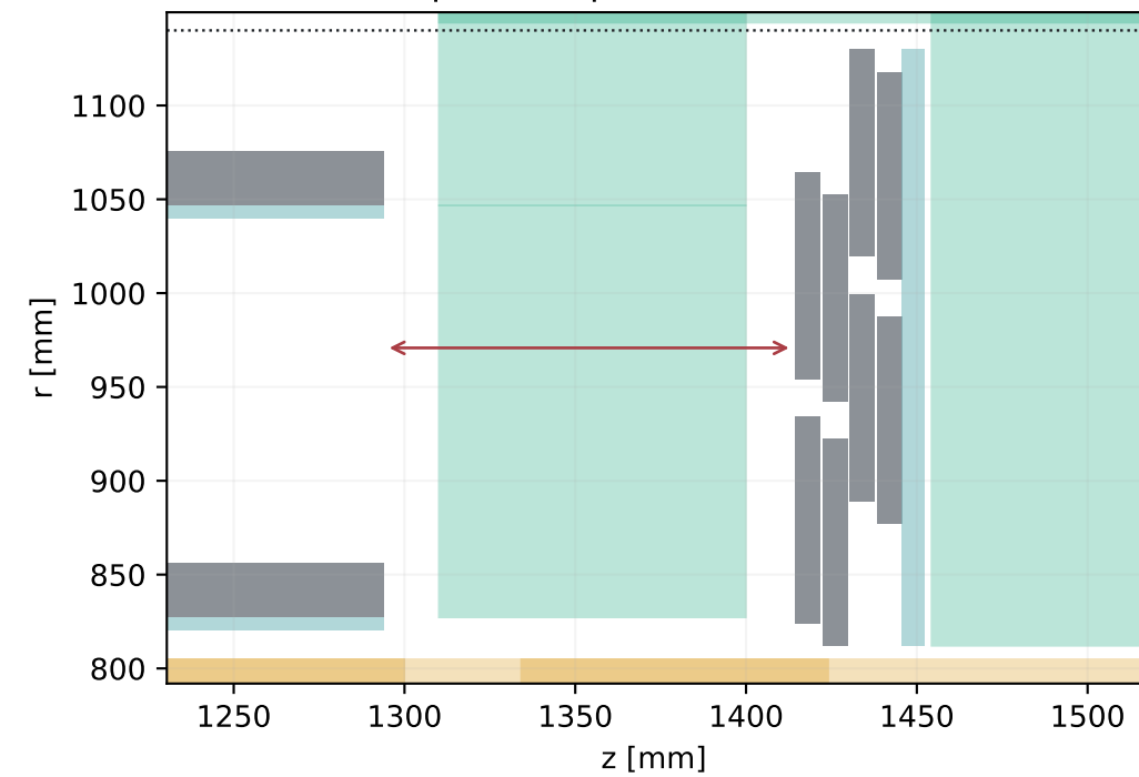
Long-strip pairs · barrel / first disc Occupied z separation: 120.56 mm
