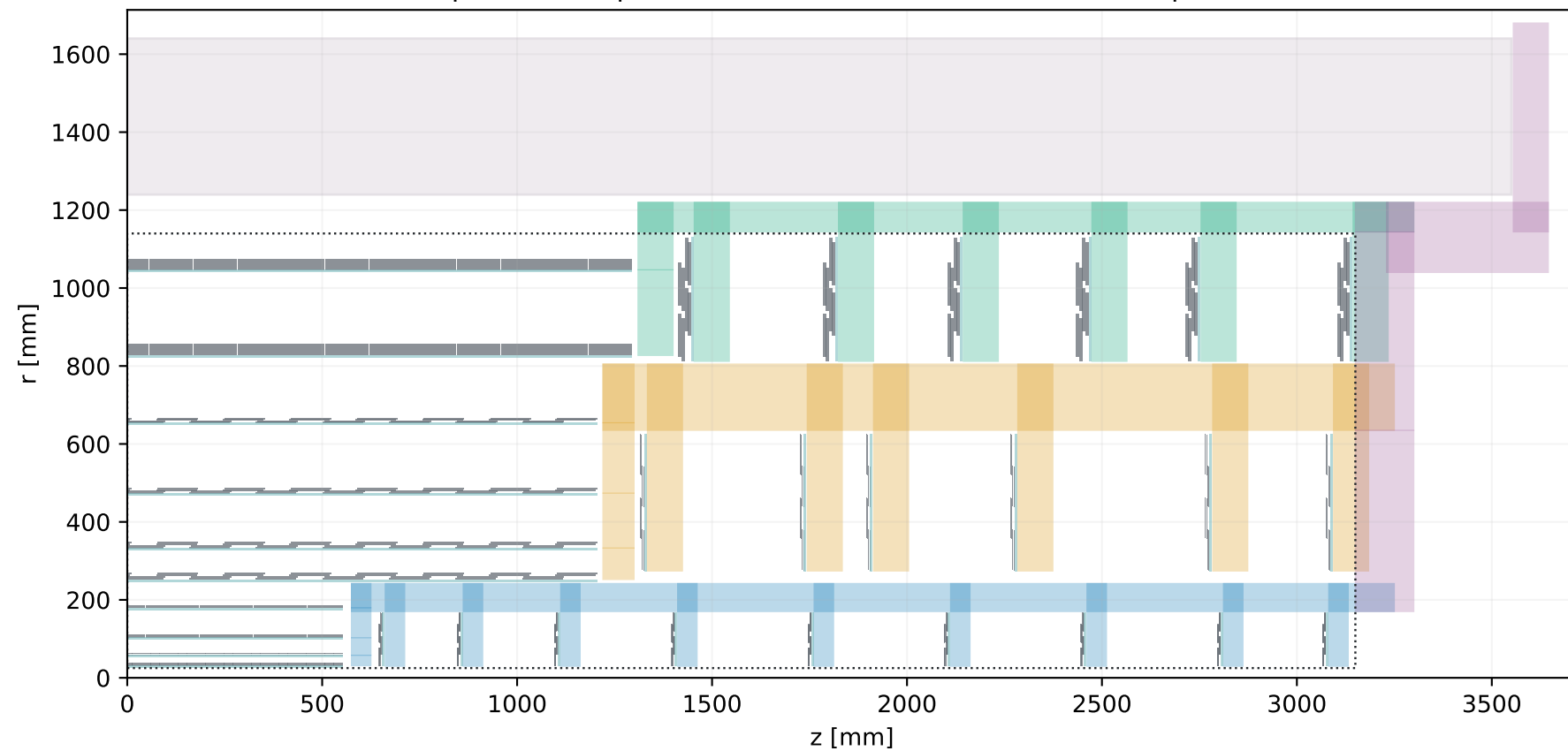
Pixels · barrel / first disc Occupied z separation: 92.50 mm
