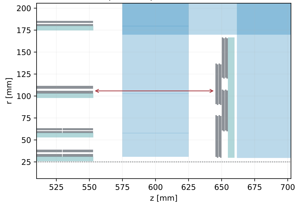
Pixels · barrel / first disc Occupied z separation: 92.50 mm
