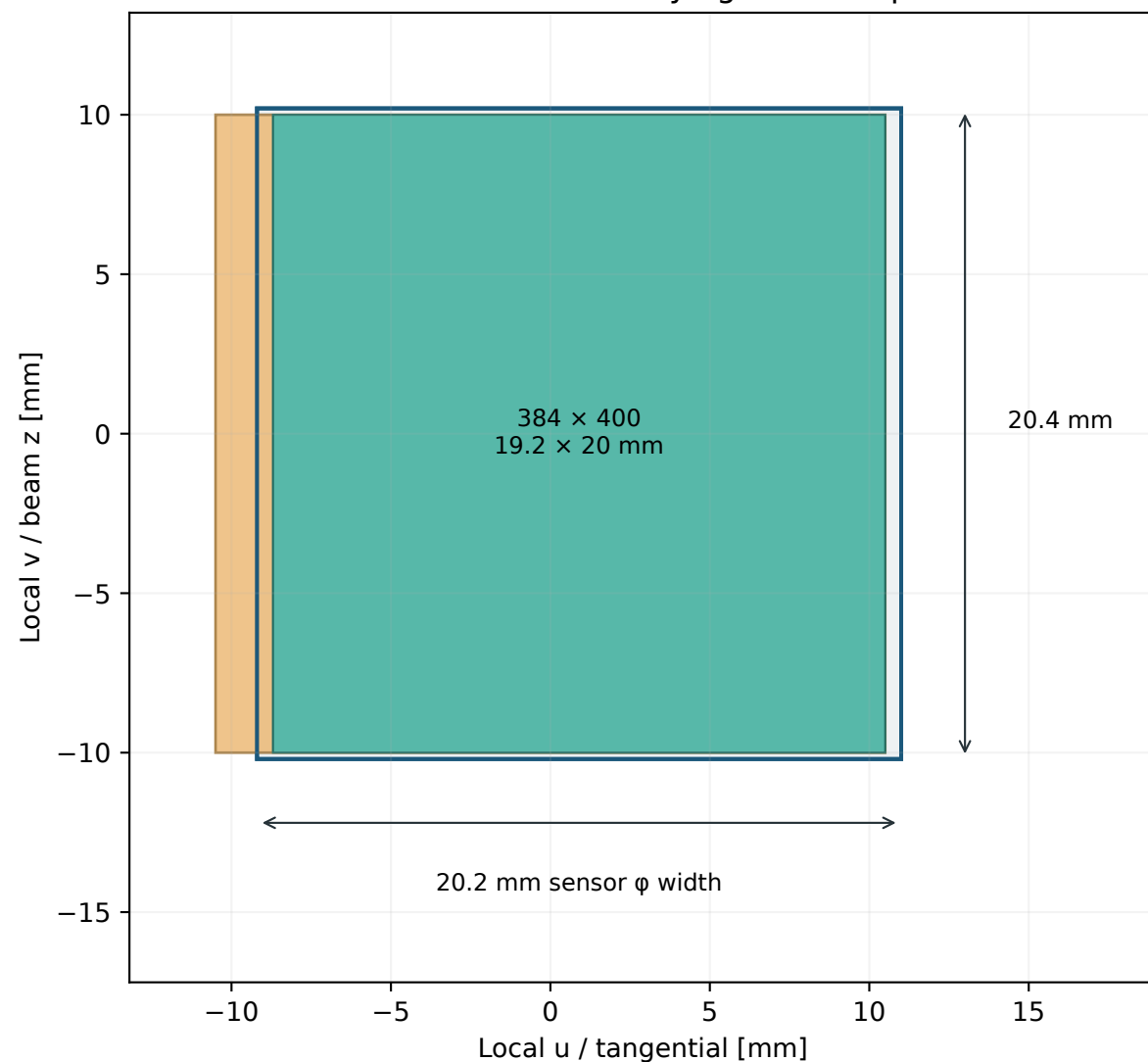
Sensor face and underlying ASIC footprints
