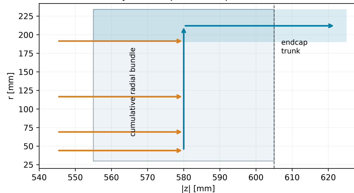
Radial bay → outer pixel endcap trunk (schematic)
