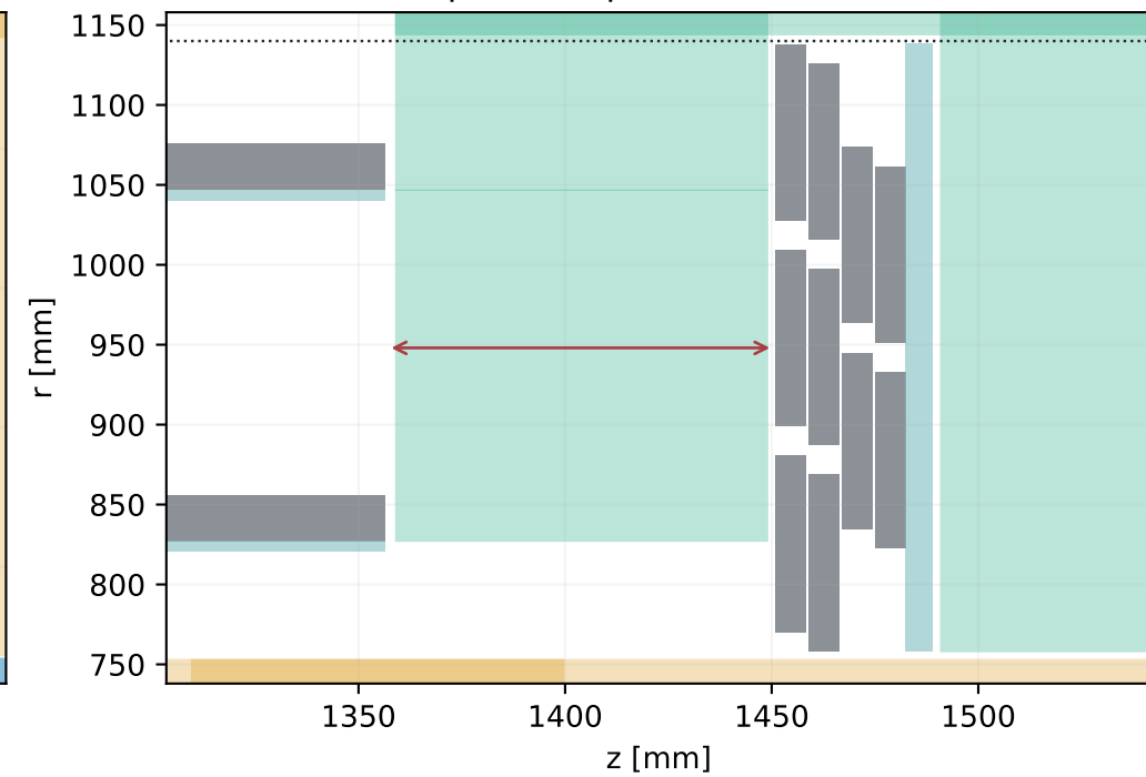
Long-strip pairs · barrel / first disc Occupied z separation: 94.54 mm
