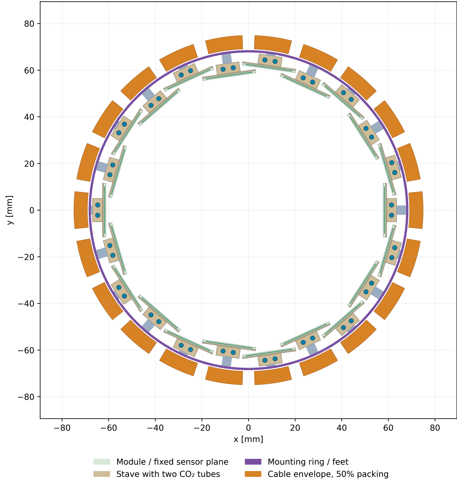
Candidate A | B2 | actual x-y cut at z = +110 mm Cumulative electrical bundles outside mounting rings
