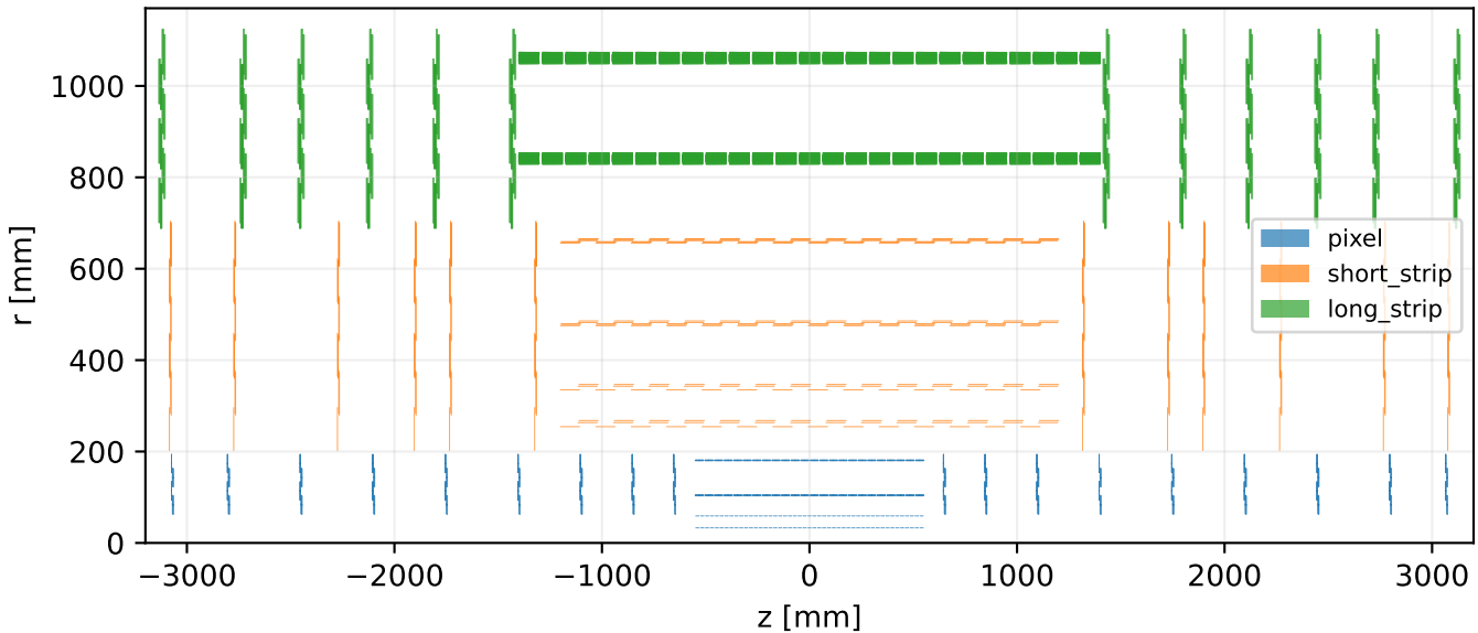
Finite active rectangles projected into r-z; |\text{module-centre } \phi| < 0.12 \text{ rad} cobe: default
