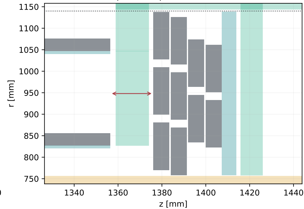
Long-strip pairs · barrel / first disc Occupied z separation: 19.54 mm
