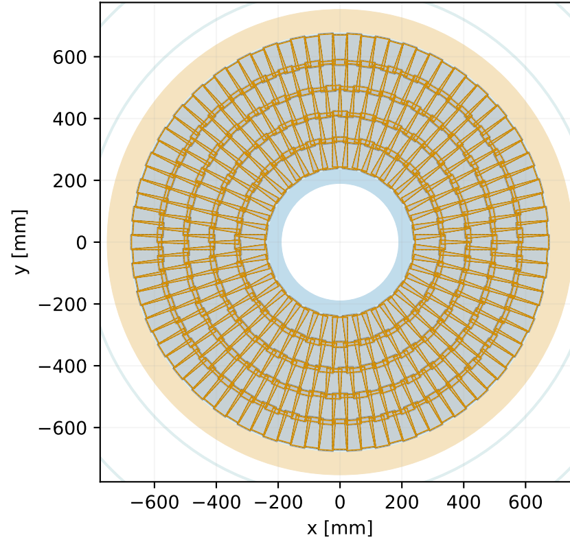
Short strips · final disc projection Nominal z = 3080 mm
