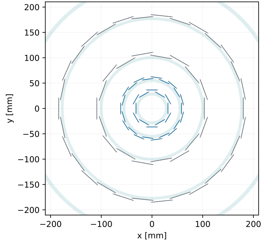
Pixels · first disc projection Nominal z = 605.7 mm
