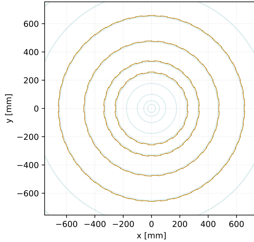
Short strips · first disc projection Nominal z = 1275.5 mm
