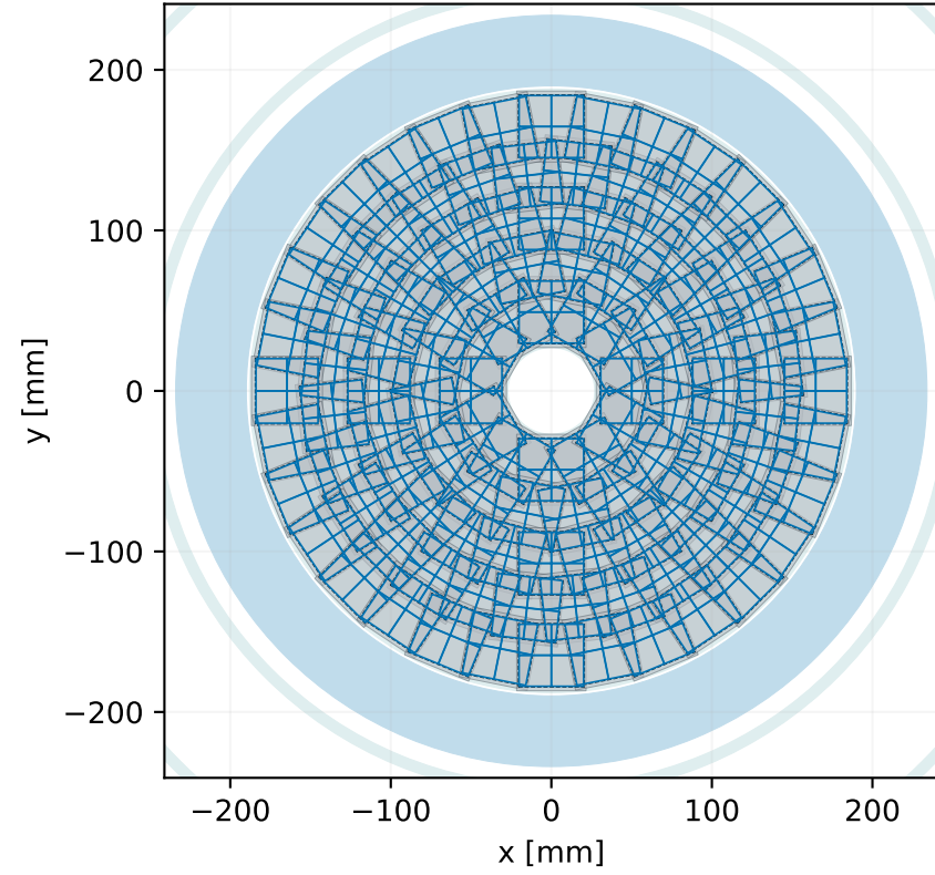
Pixels · final disc projection Nominal z = 3070 mm
