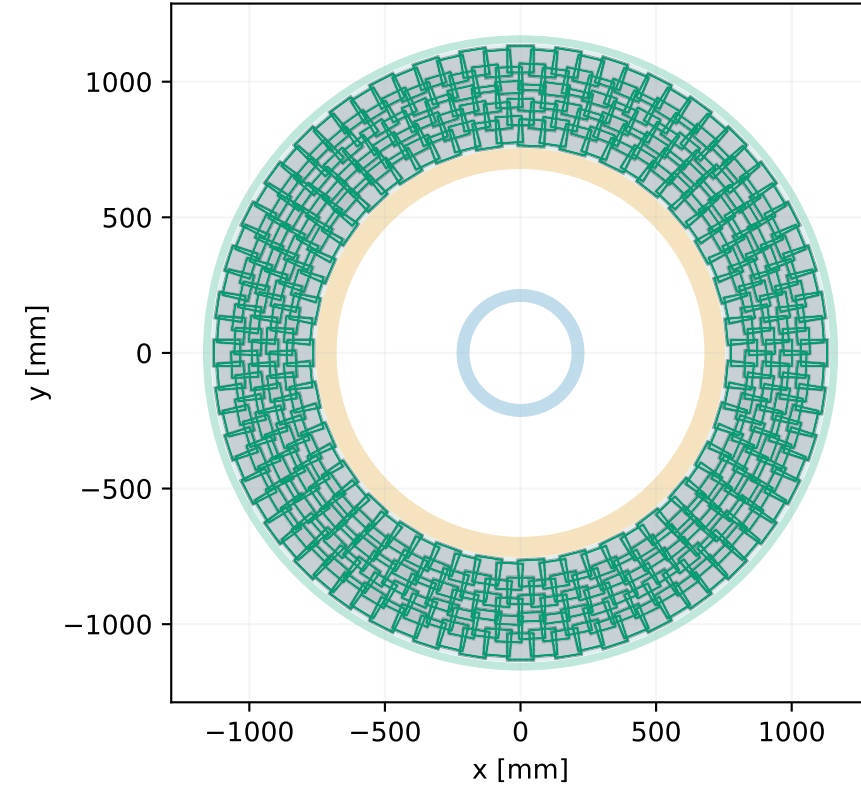
Long-strip pairs · final disc projection Nominal z = 3120 mm
