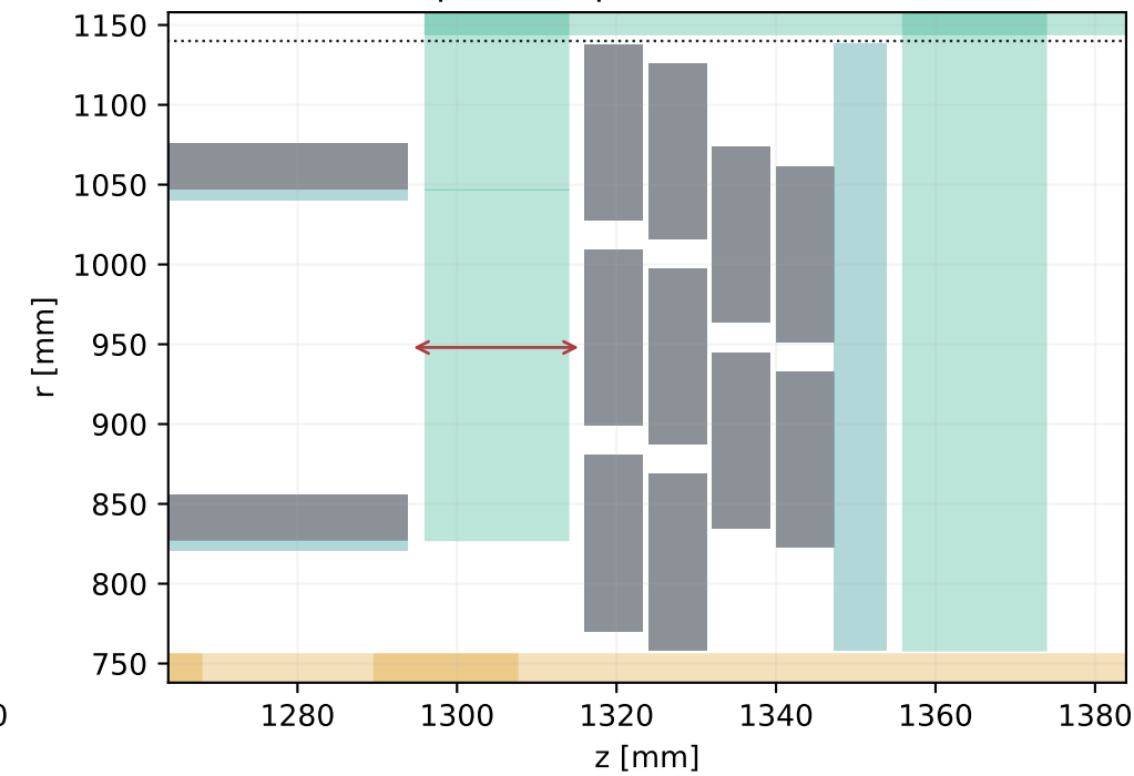
Long-strip pairs · barrel / first disc Occupied z separation: 22.21 mm
