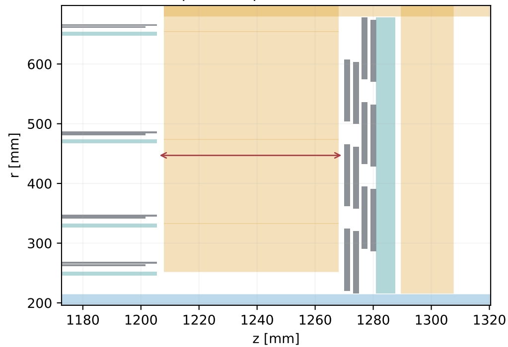
Short strips · barrel / first disc Occupied z separation: 64.50 mm
