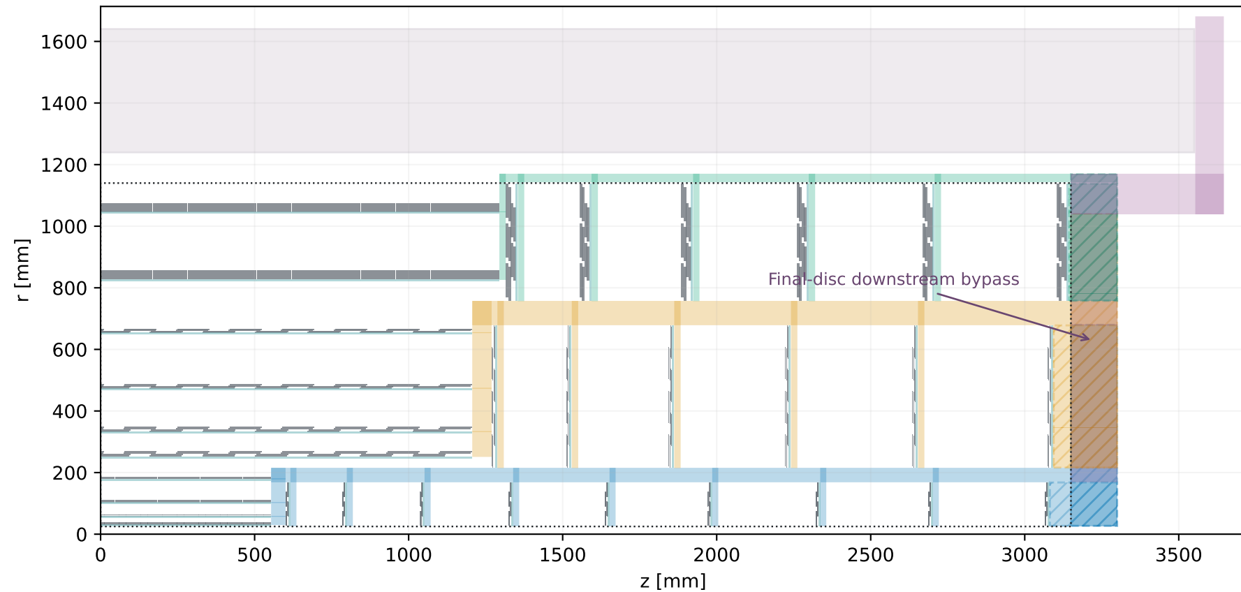
Pixels · barrel / first disc Occupied z separation: 48.20 mm
