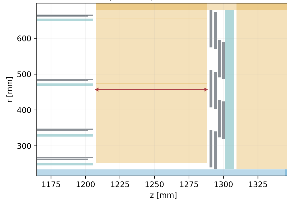
Short strips · barrel / first disc Occupied z separation: 84.50 mm
