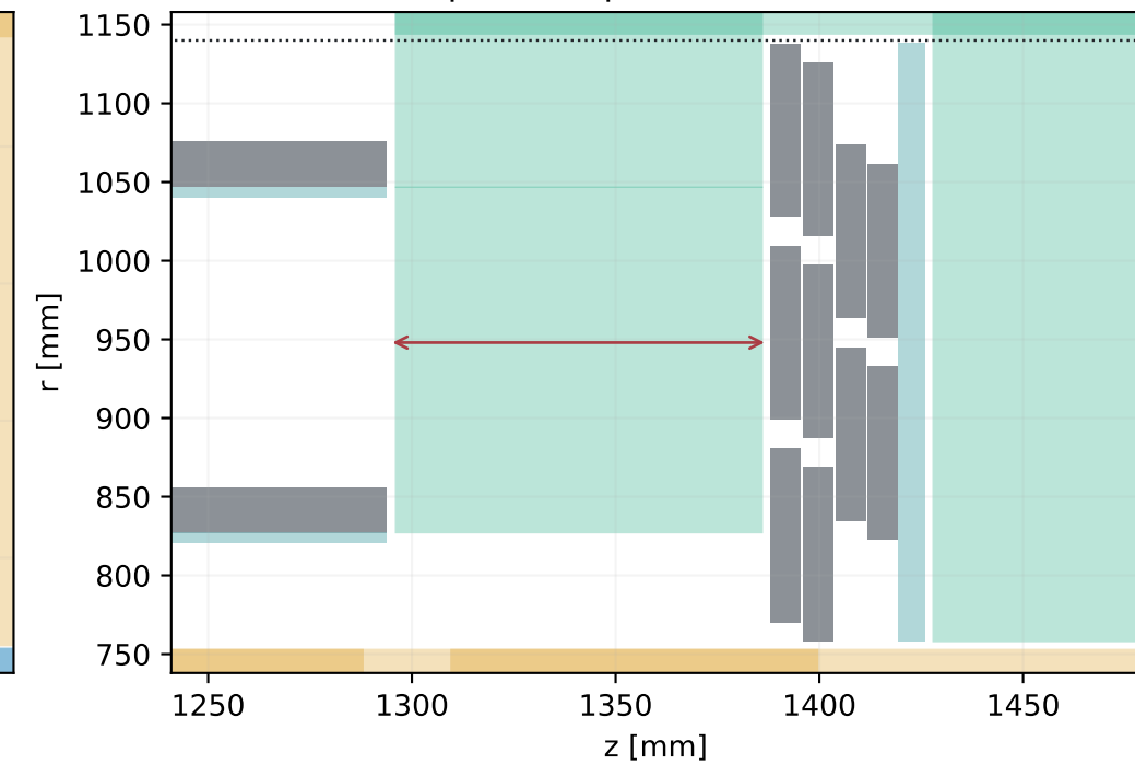
Long-strip pairs · barrel / first disc Occupied z separation: 94.21 mm
