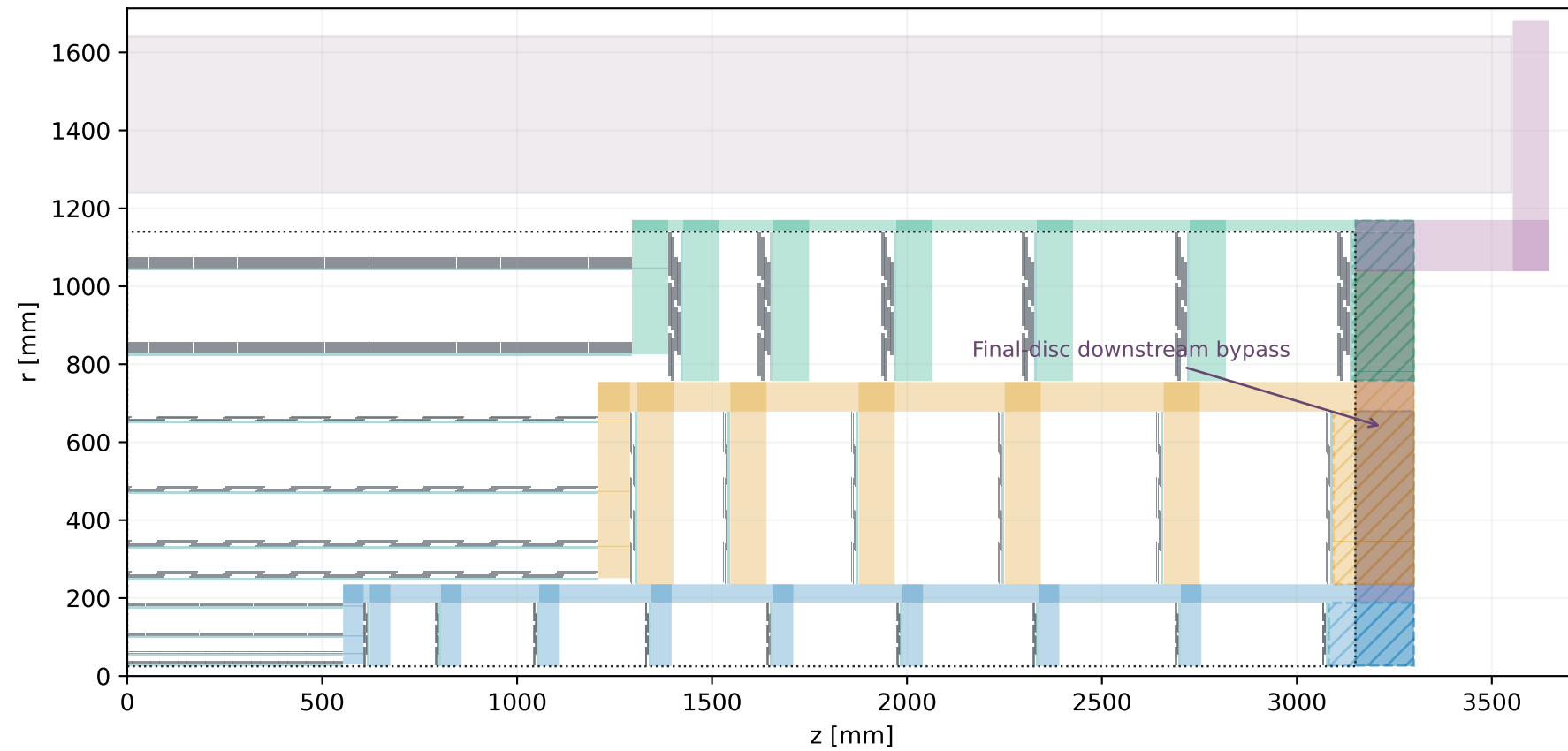
Pixels · barrel / first disc Occupied z separation: 54.20 mm
