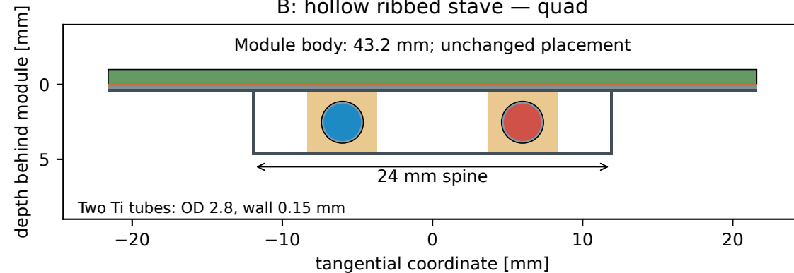
B: hollow ribbed stave — quad
