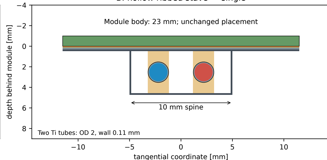
B: hollow ribbed stave — single
