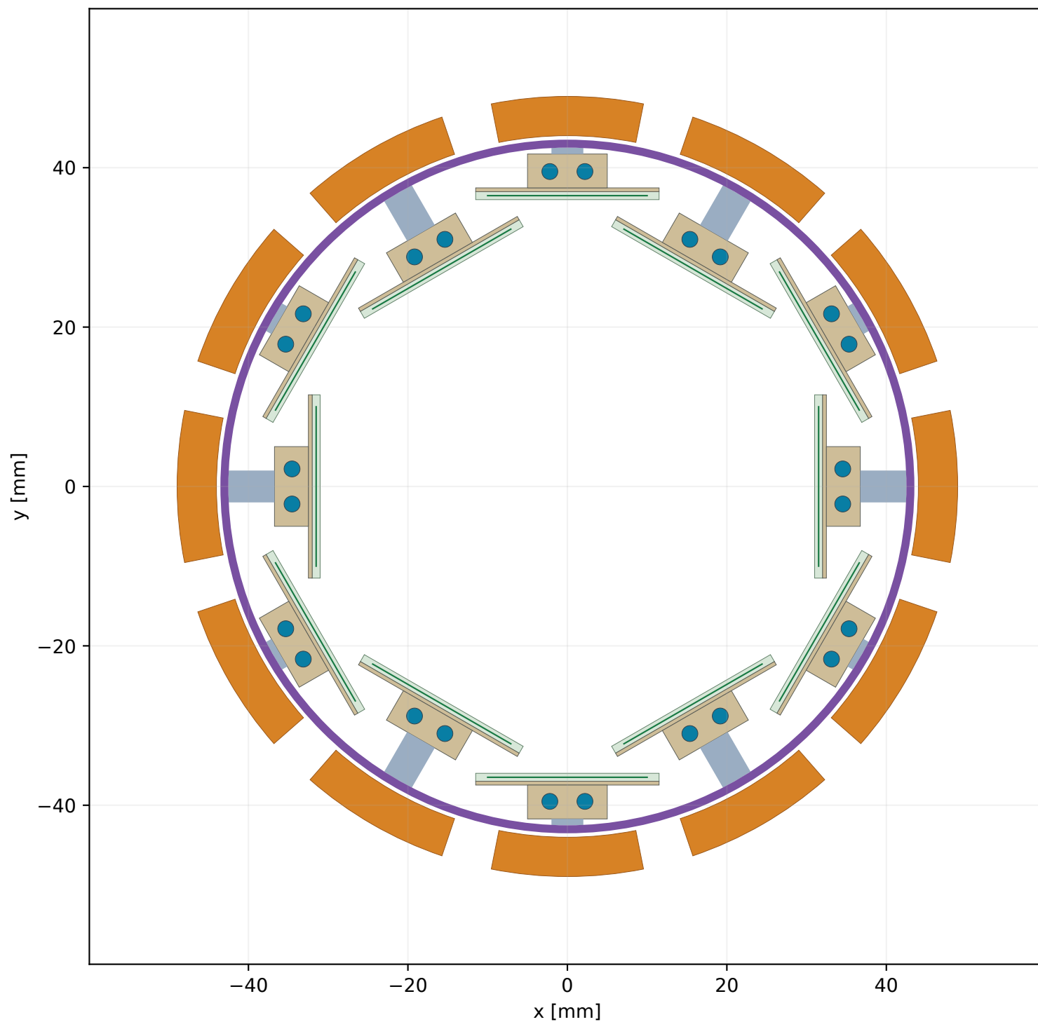
Candidate A | B1 | actual x-y cut at z = +110 mm Cumulative electrical bundles outside mounting rings
