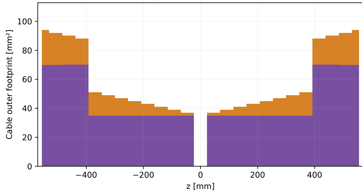
B4 | one stave, both exits
