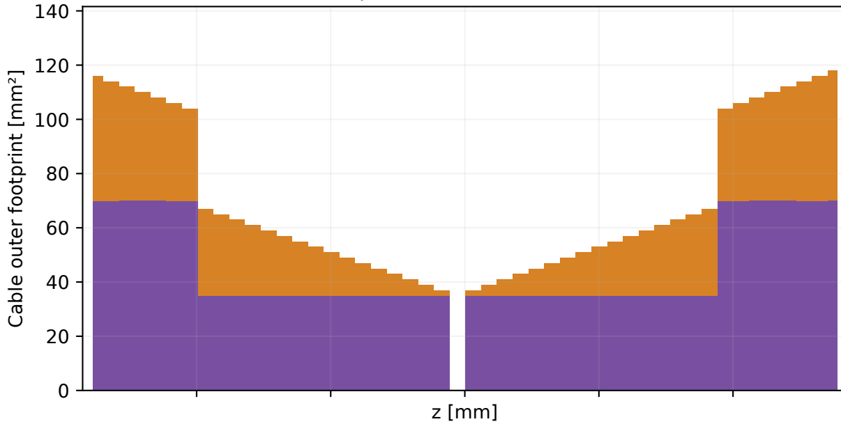
B3 | one stave, both exits
