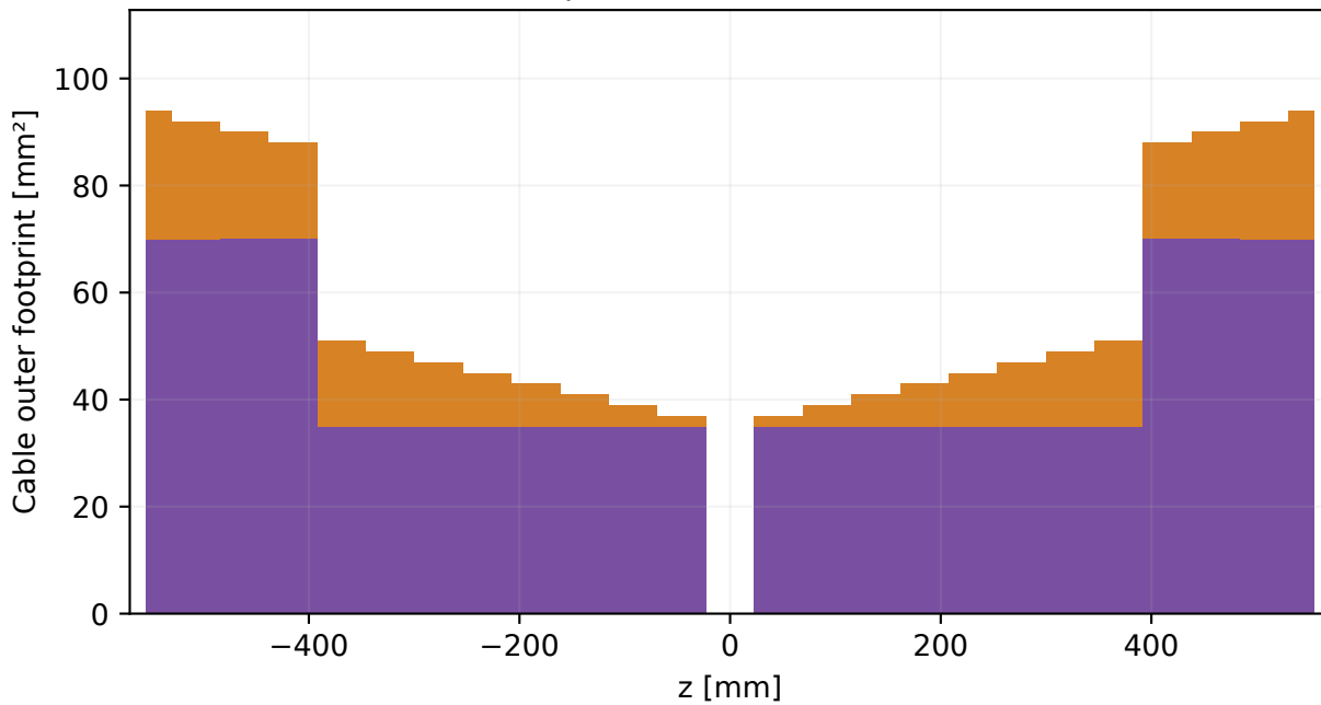
B3 | one stave, both exits
