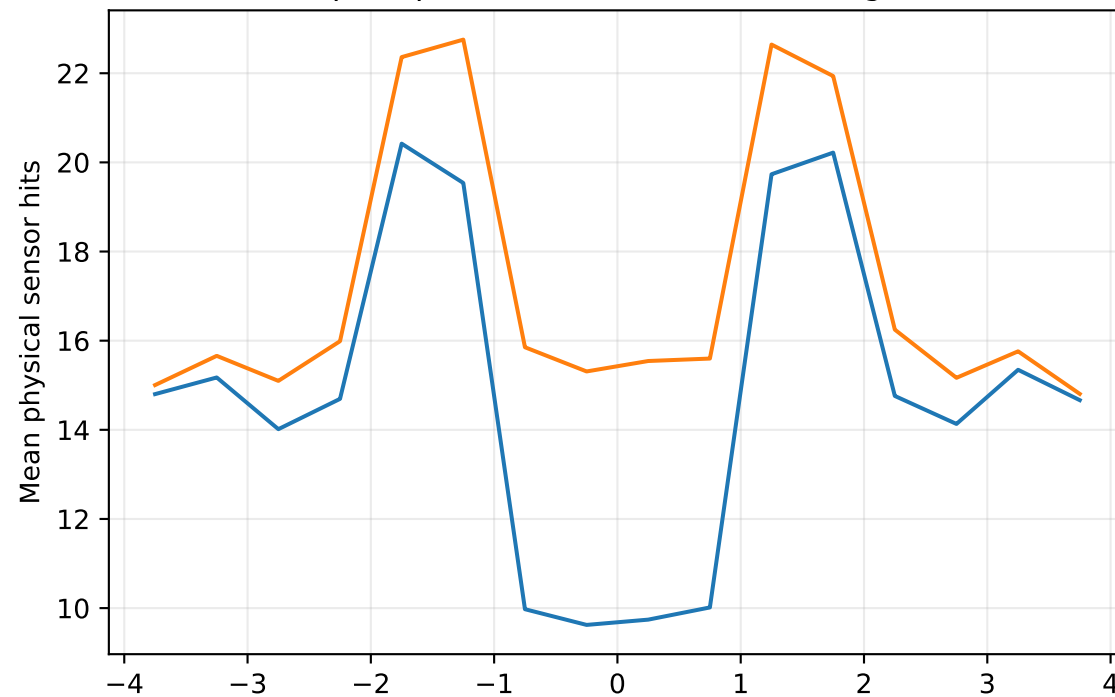
pint: p = 1 GeV, B_z = 3 T, + charge
