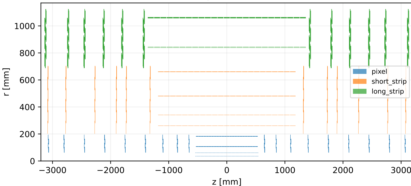
pint: hybrid clearance
