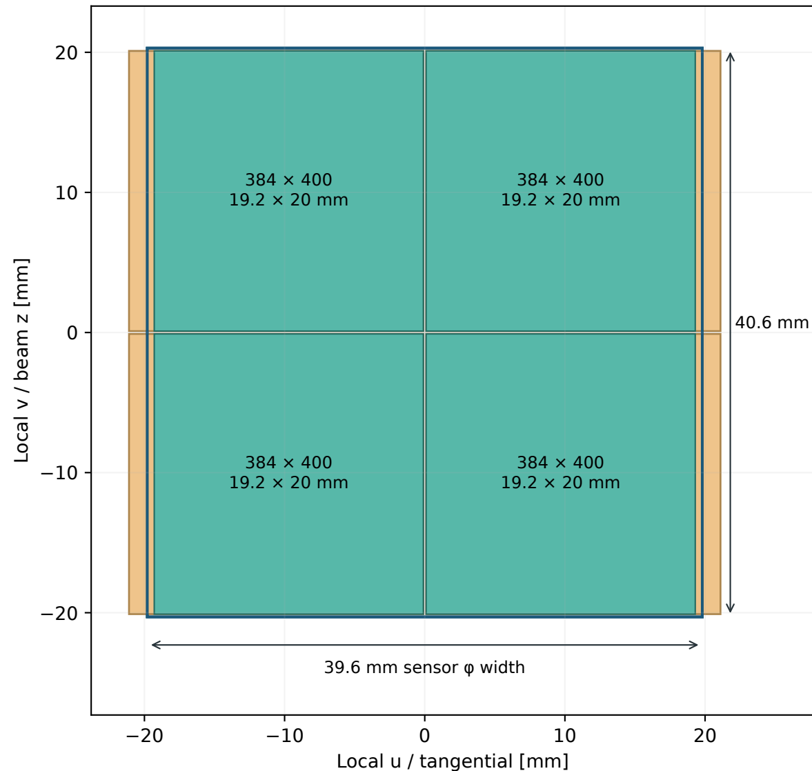
Sensor face and underlying ASIC footprints
