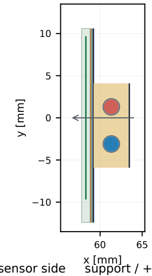
B2 stave detail (same x-y axes)
