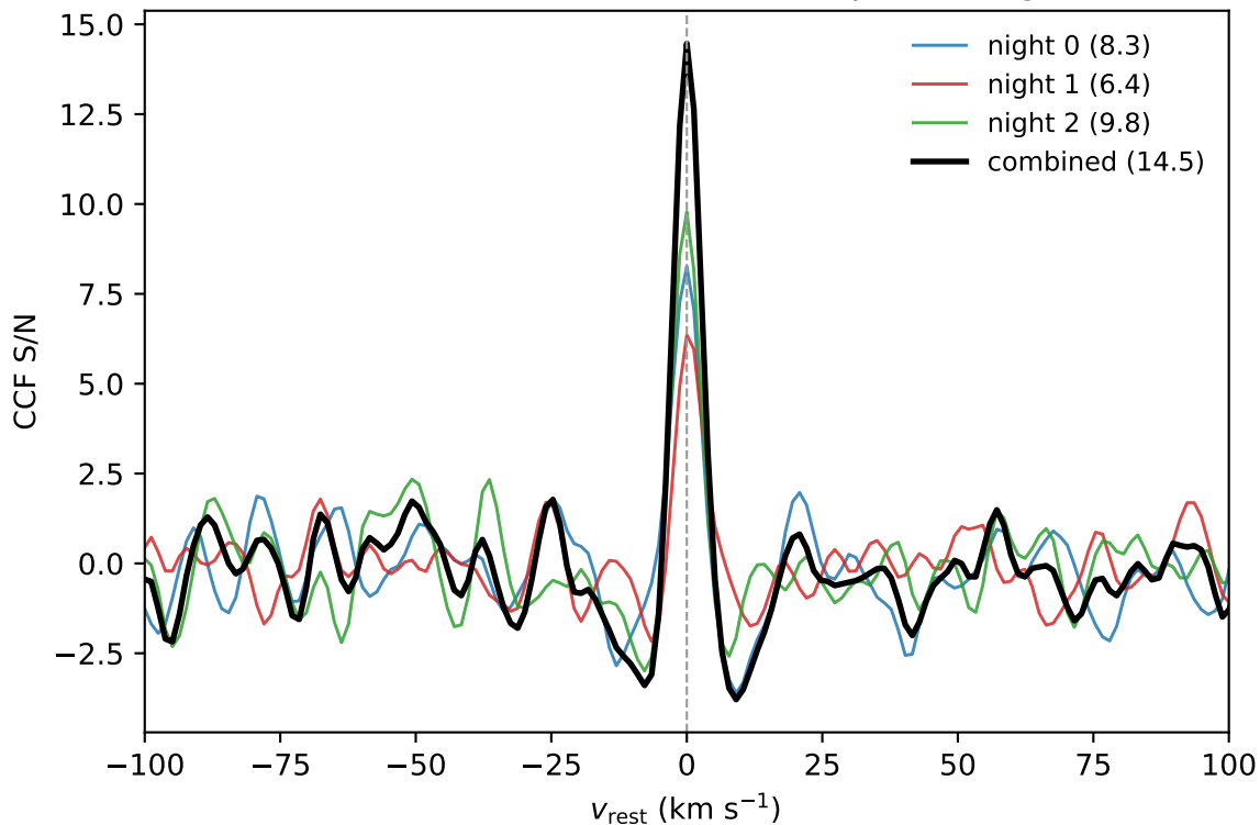
CARMENES NIR (3.5 m): three repeated nights
