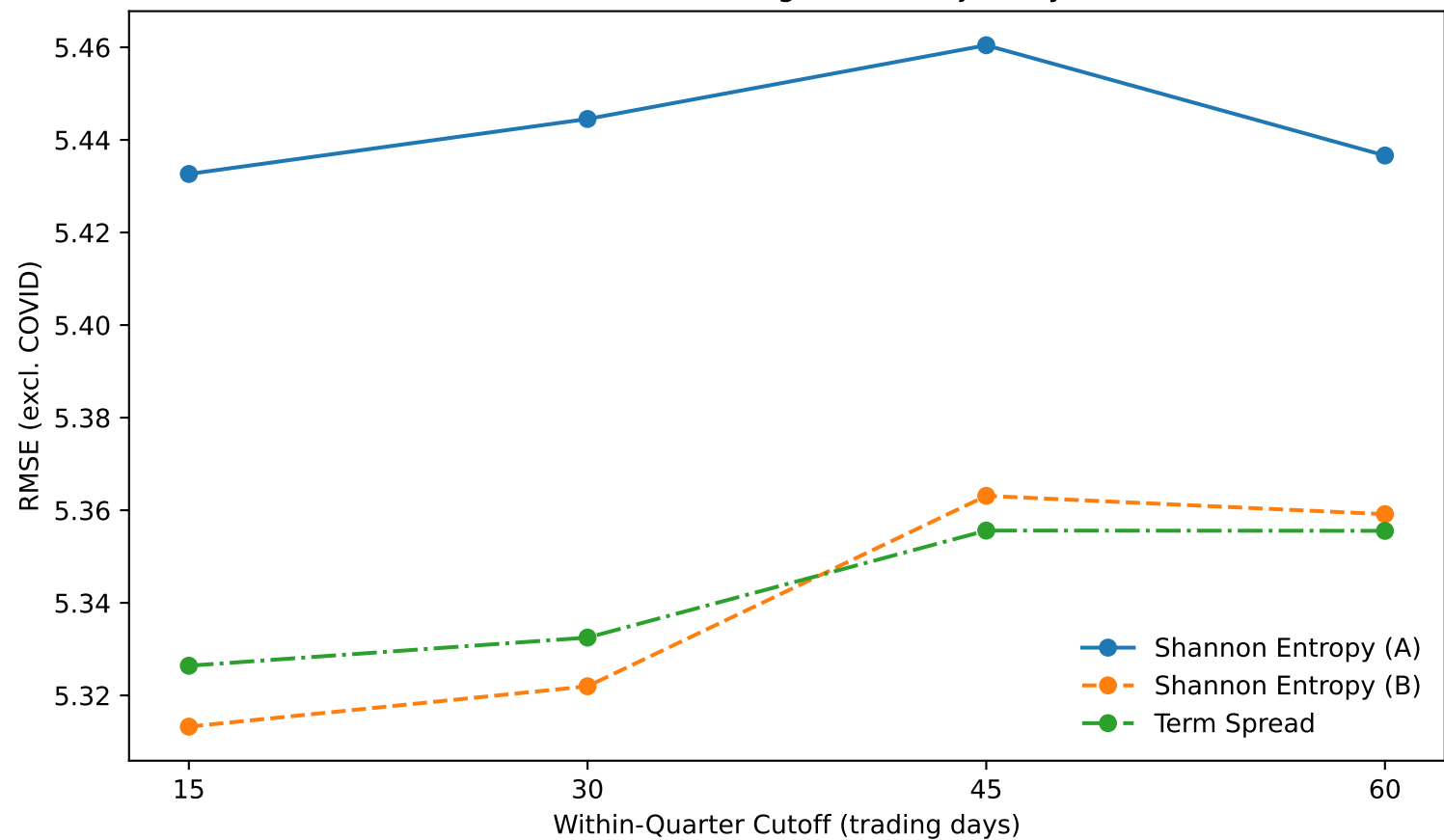
MIDAS Nowcasting: RMSE Trajectory
