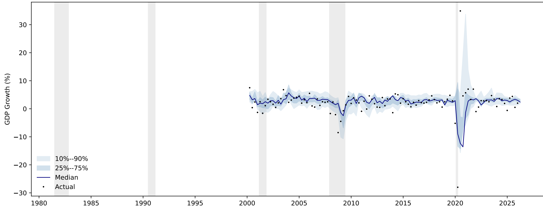
Quantile Fan Chart — Spec (2) A , h = 1
