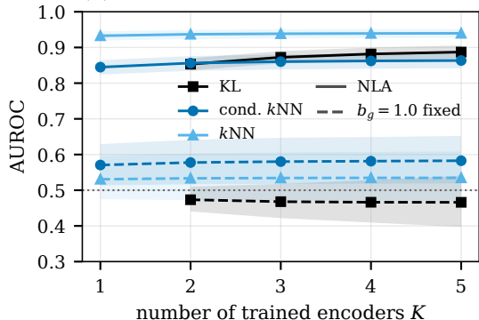
(b) Cost: AUROC vs. number of encoders
