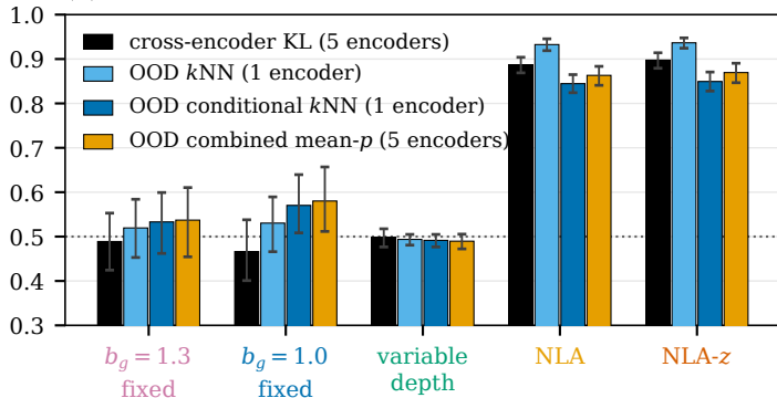
(a) Detector head-to-head
